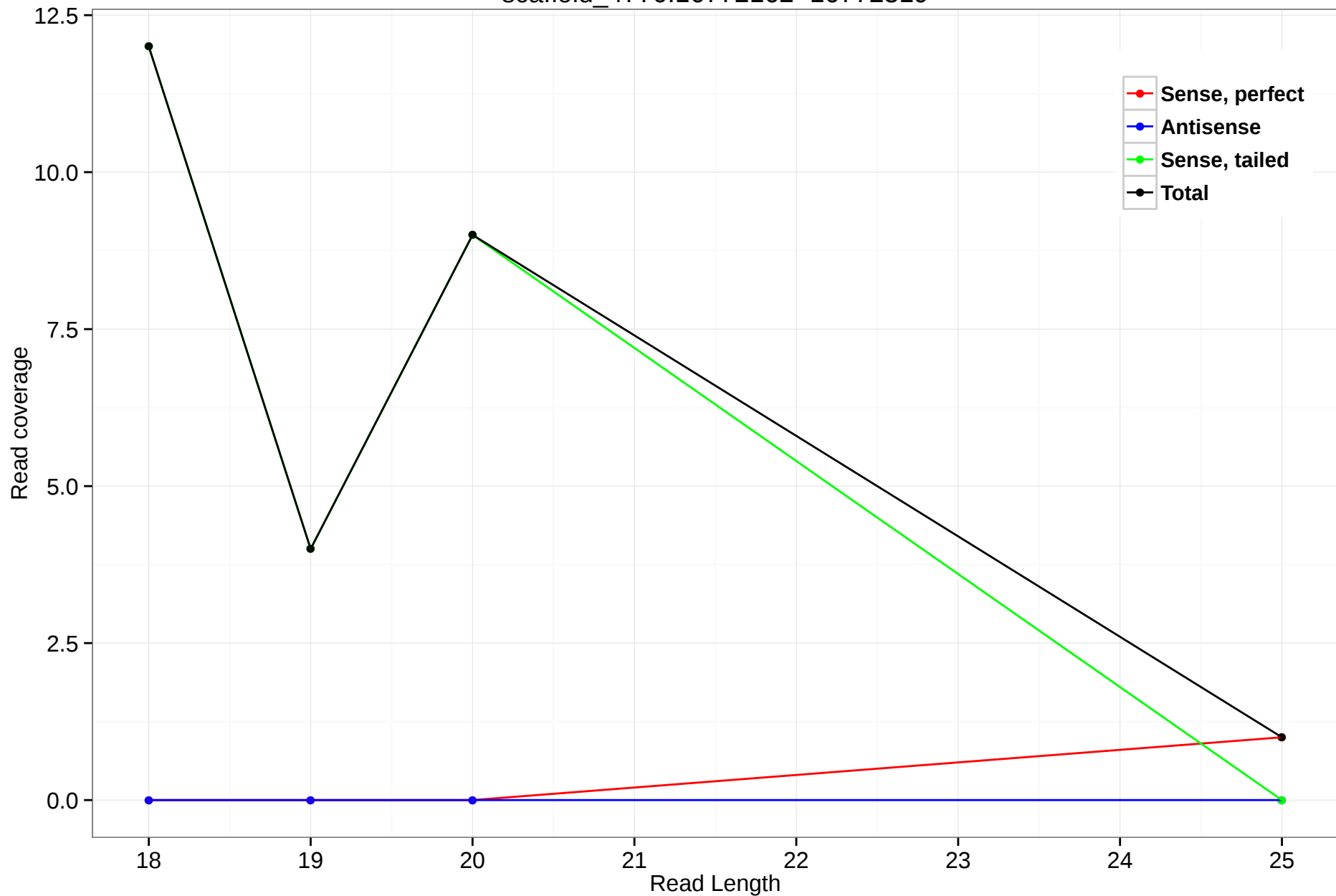
scaffold_4770:16772162-16772319
