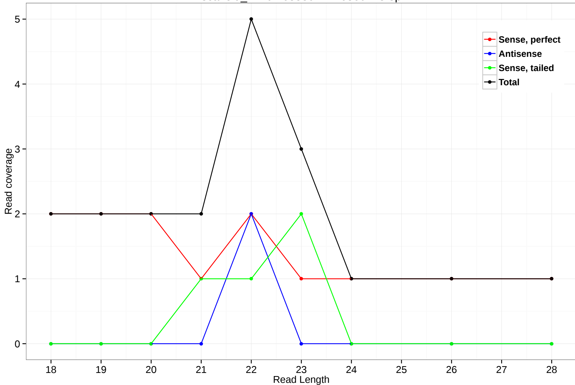
scaffold_4770:16358041-16360118.3p
