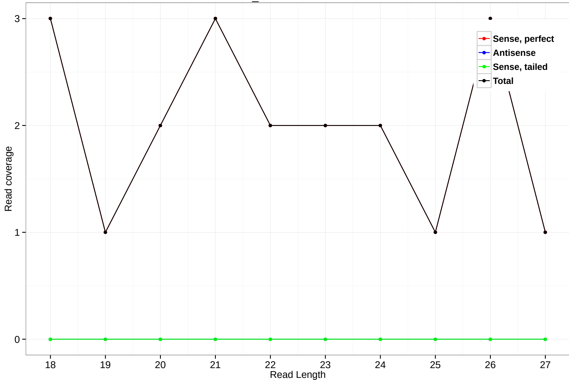
scaffold_4770:1595354-1595767
