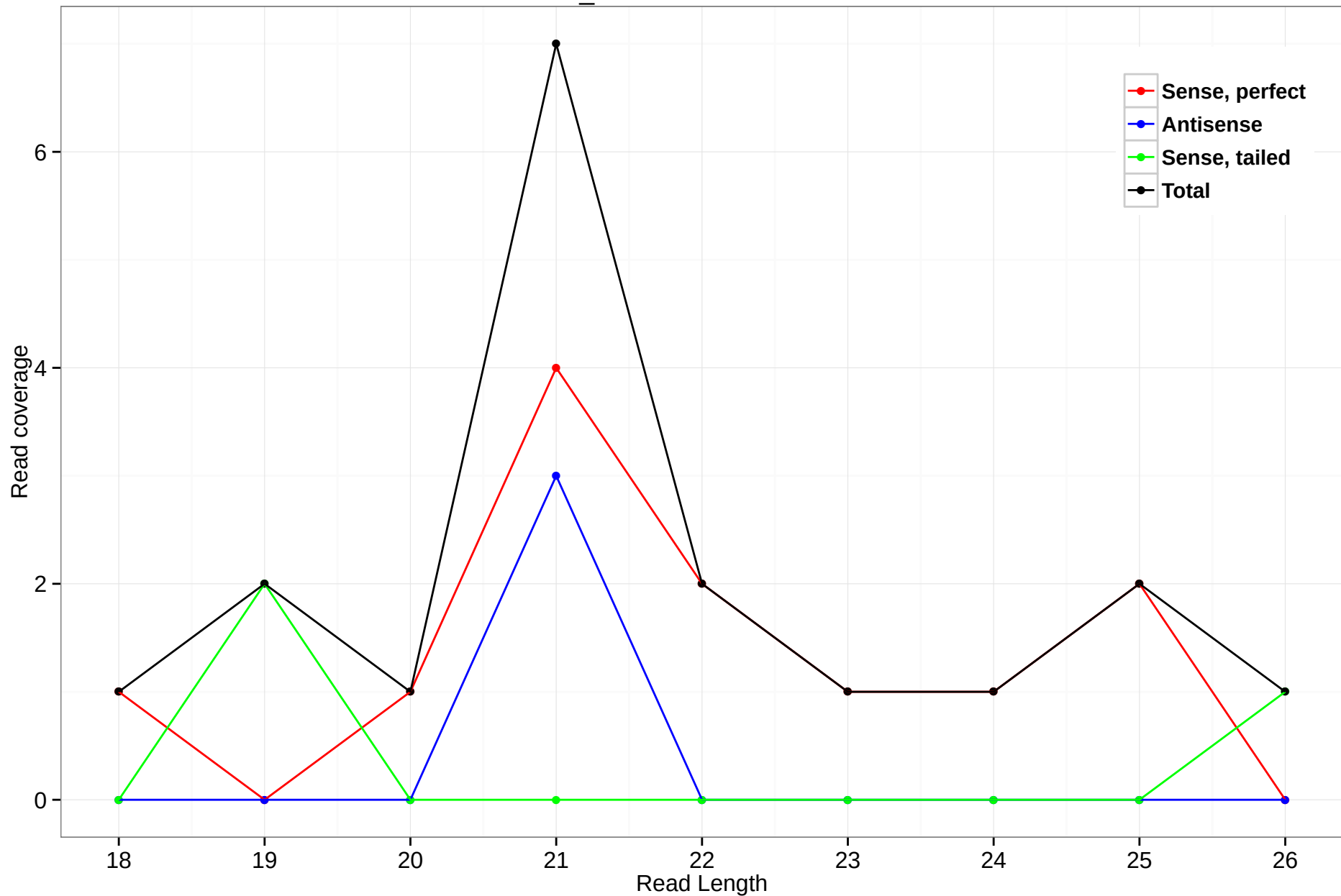
scaffold_4770:15011621-15012102
