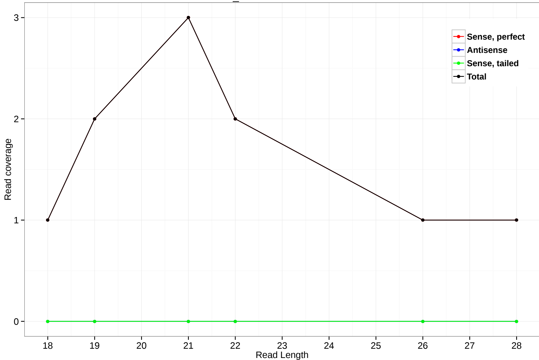
scaffold_4770:12825832-12826047
