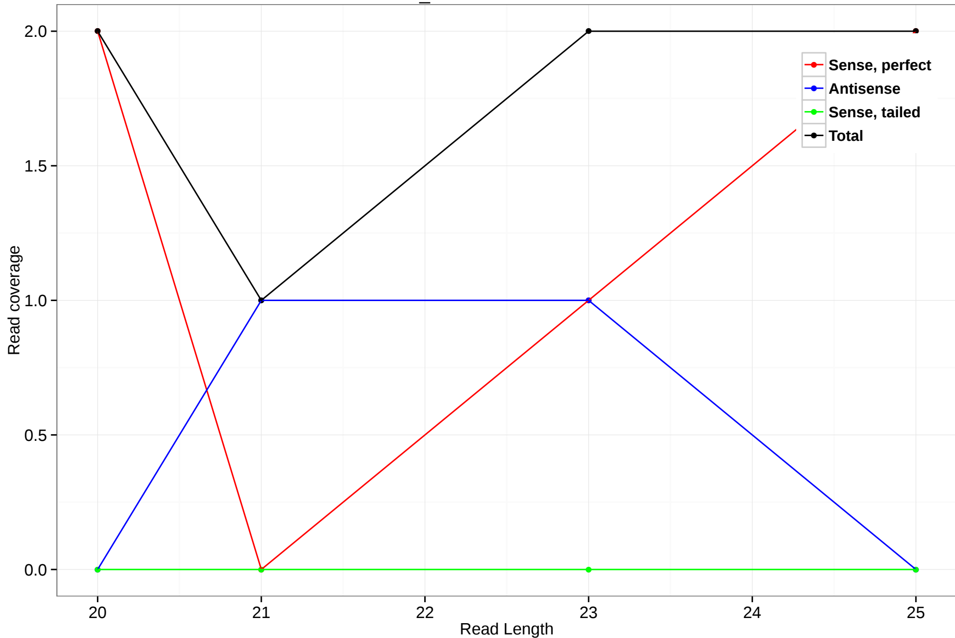
scaffold_4770:11811801-11812288
