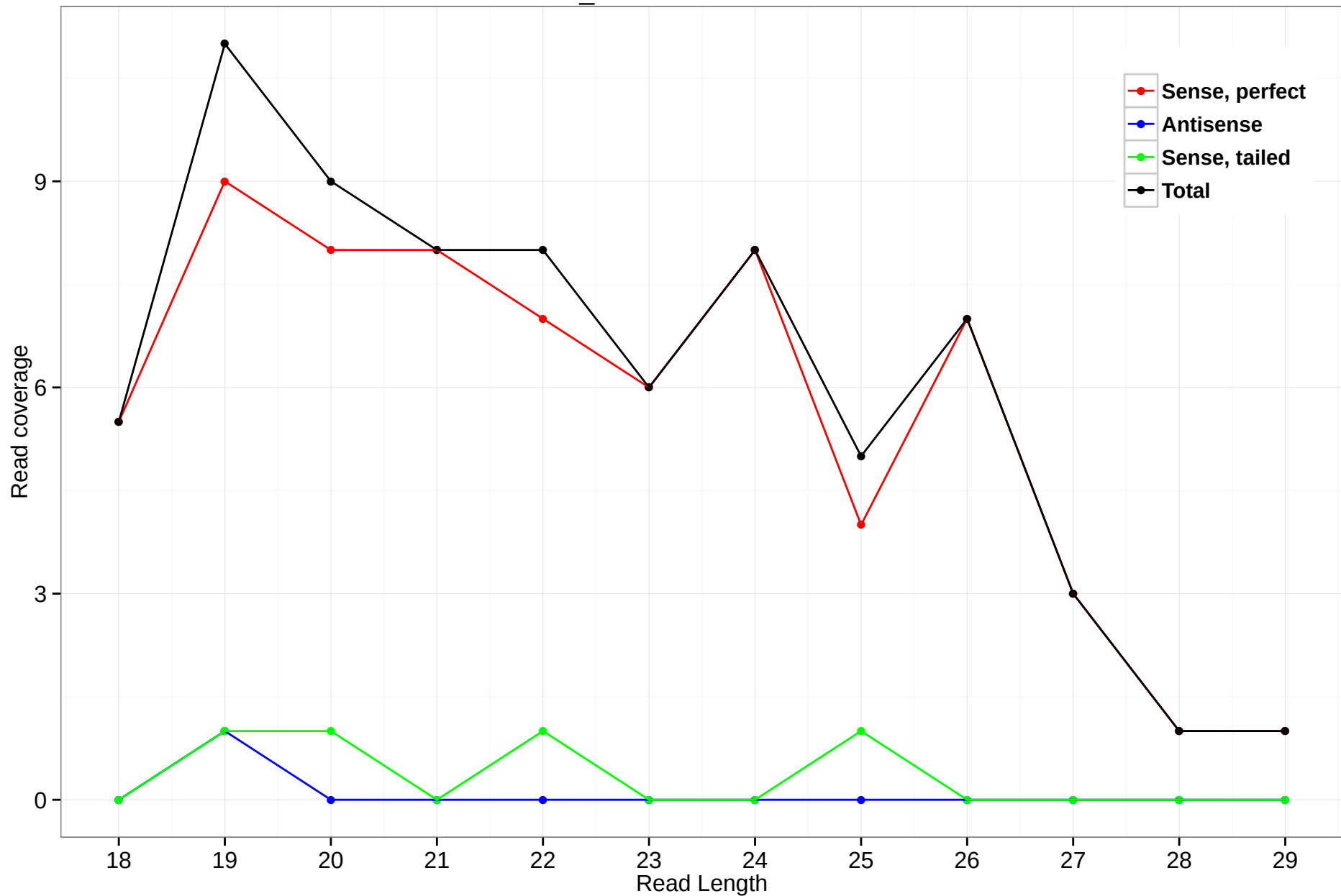
scaffold_4770:11808823-11809415
