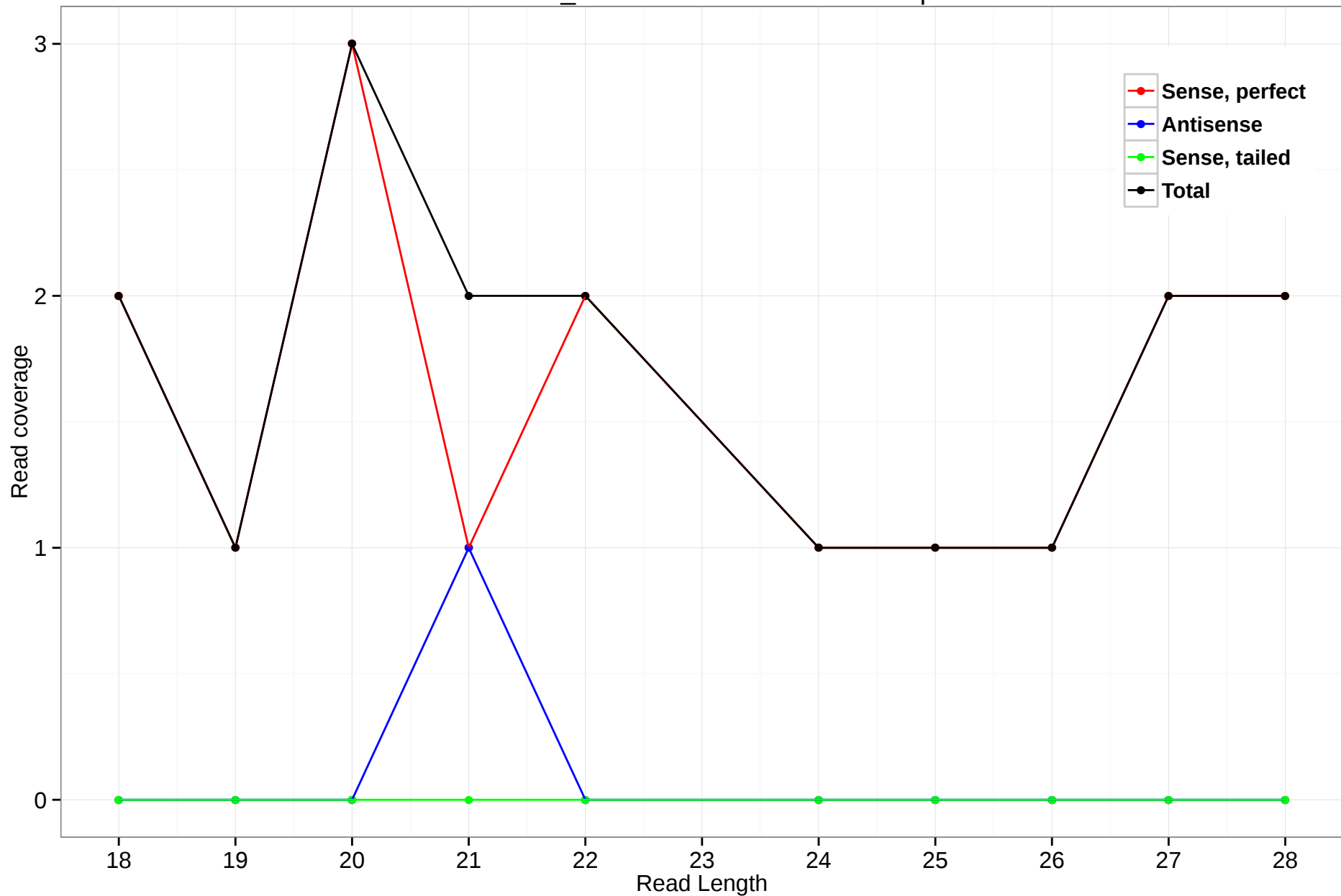
scaffold_4770:11623291-11624935.3p
