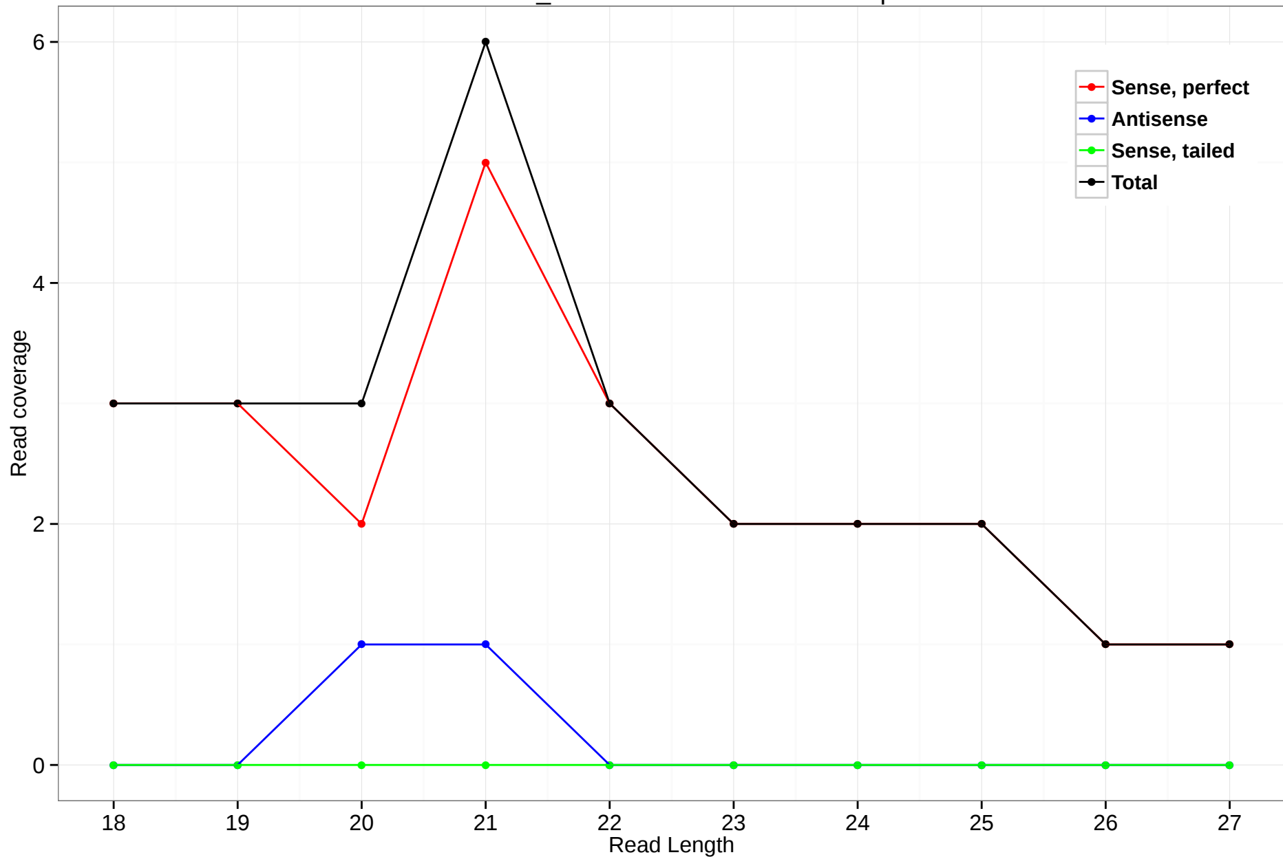
scaffold_4770:11448649-11450391.5p
