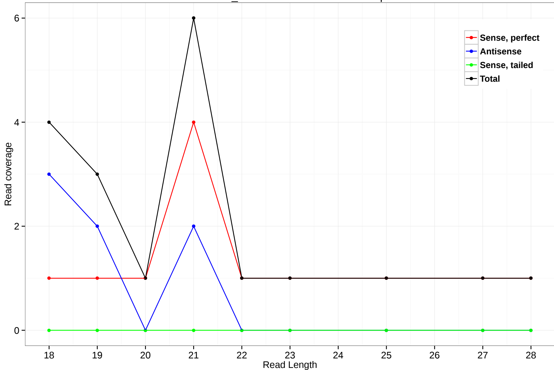
scaffold_4770:10756927-10758933.5p
