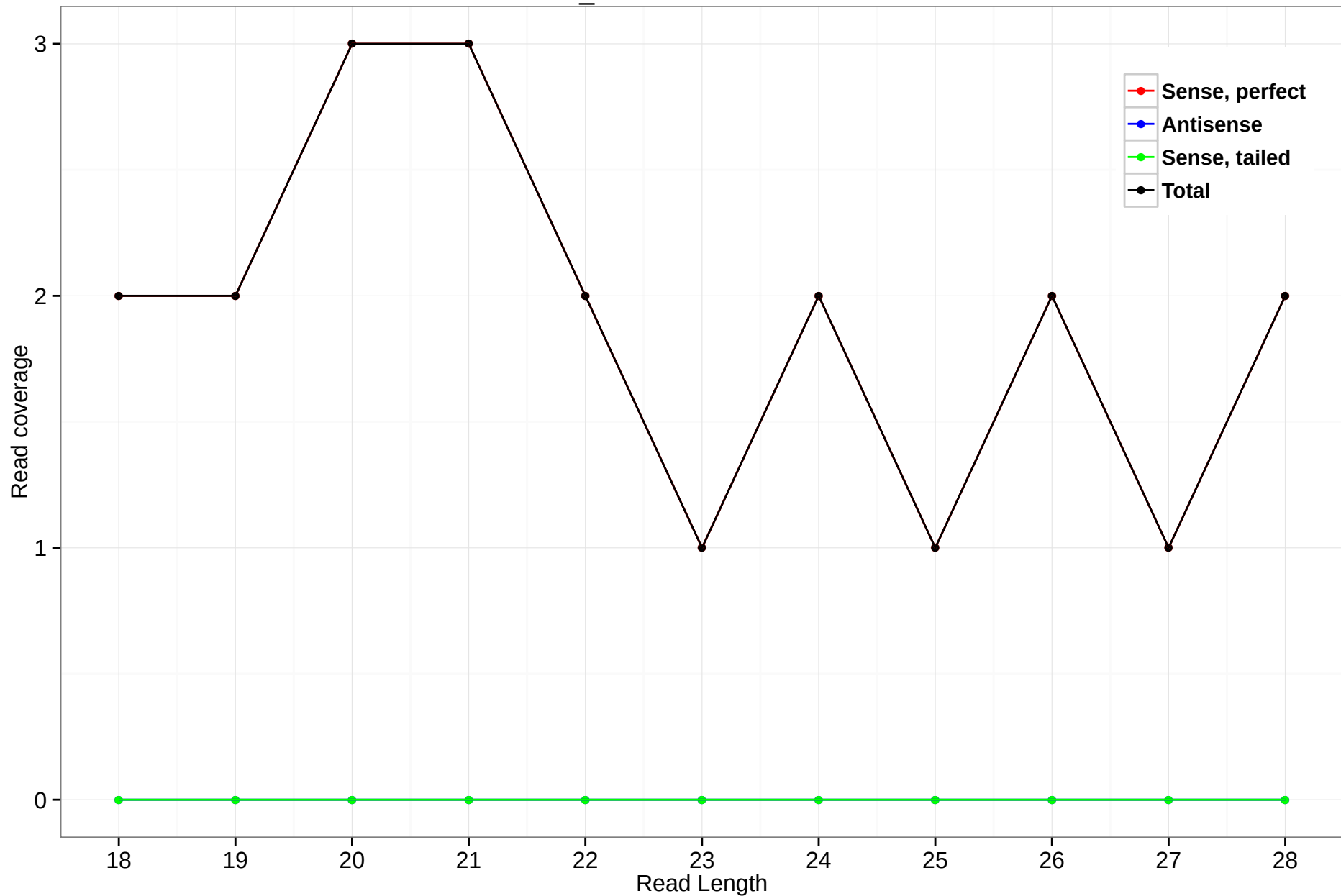
scaffold_4770:10697091-10697265
