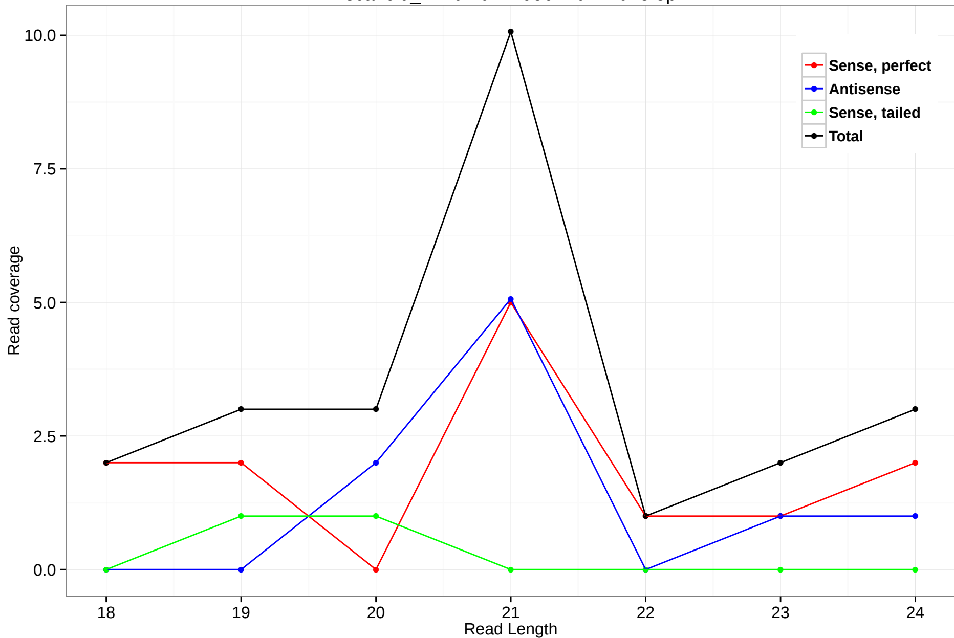
scaffold_4770:10441956-10444078.3p
