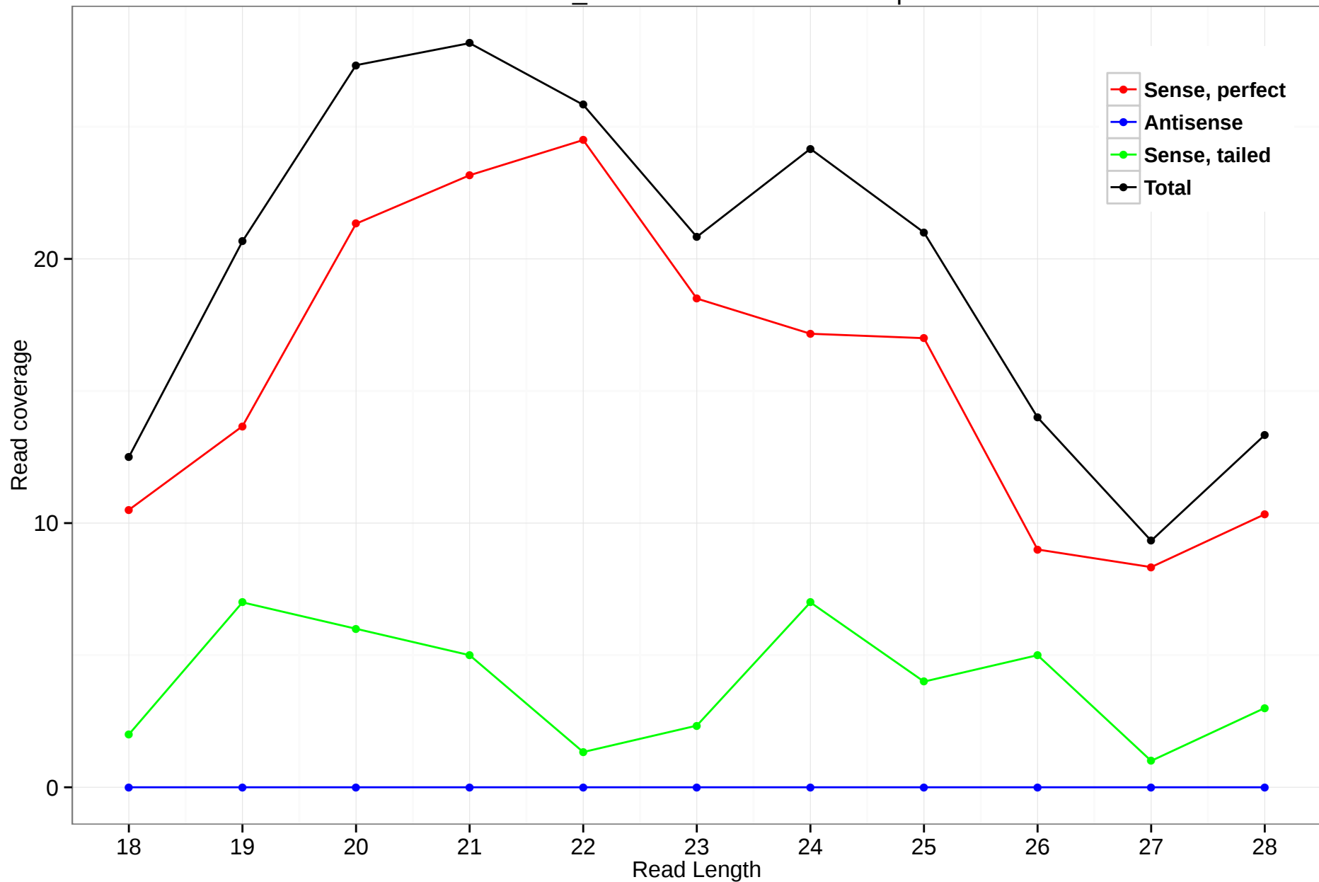
scaffold_4690:7384899-7385776.5p
