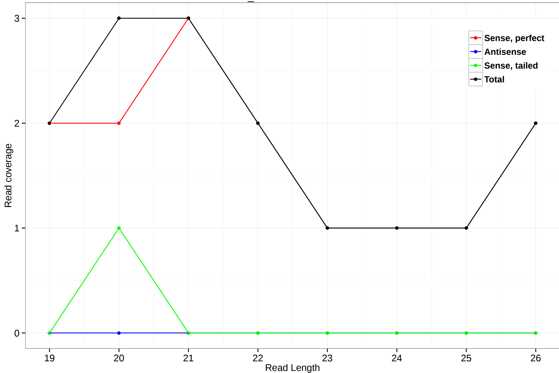
scaffold_4690:6936743-6936915
