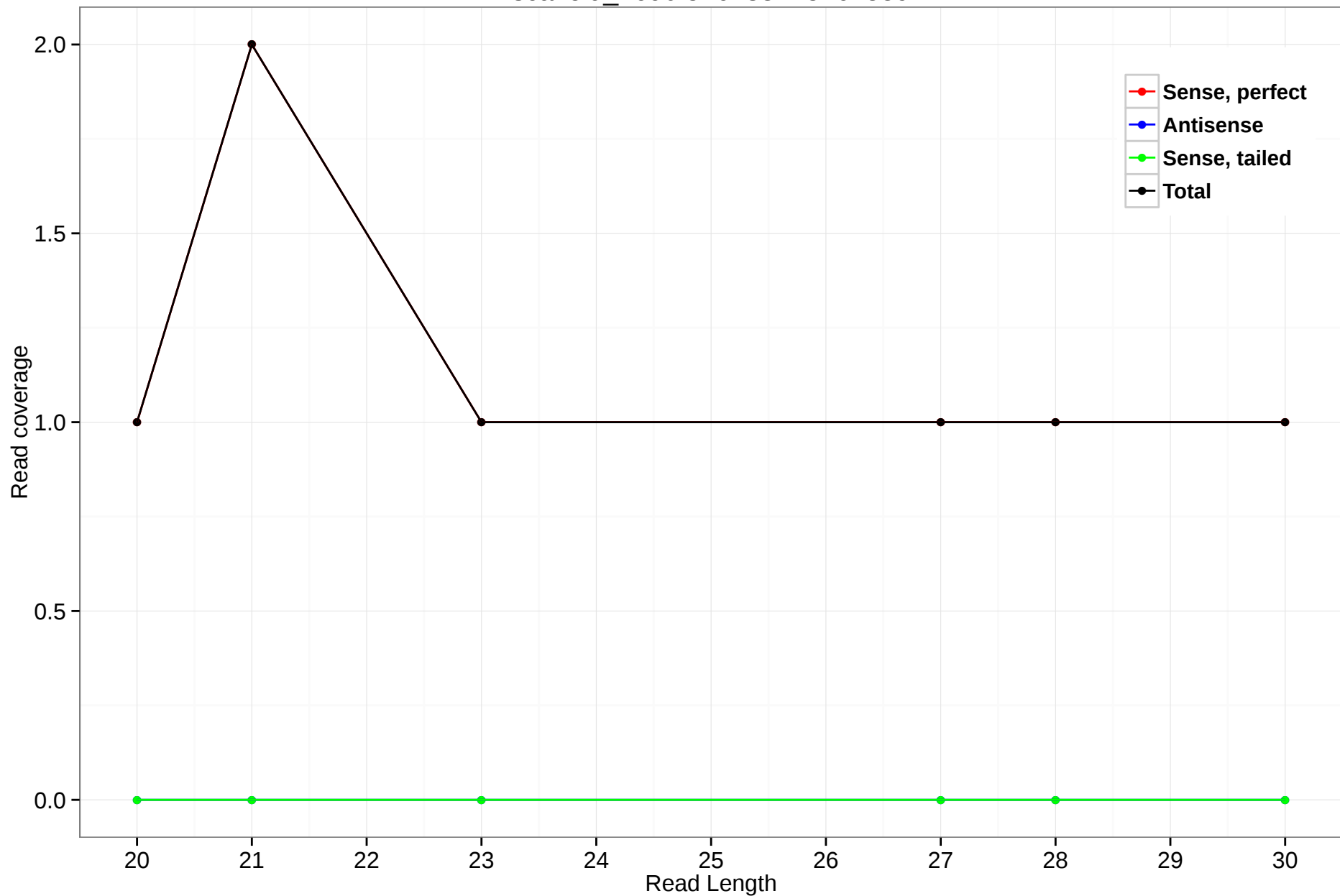
scaffold_4690:5161387-5161559
