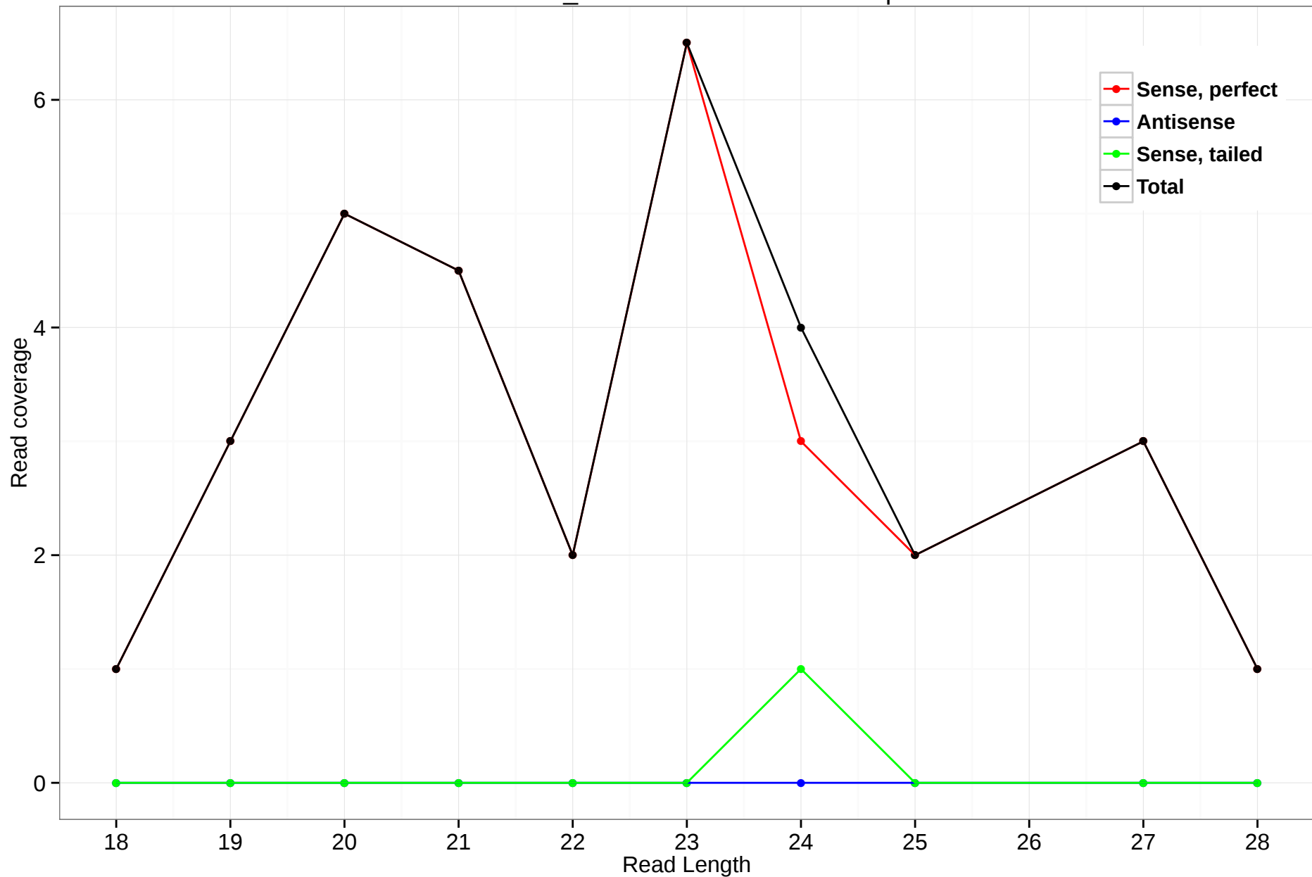
scaffold_4690:4360325-4364202.3p
