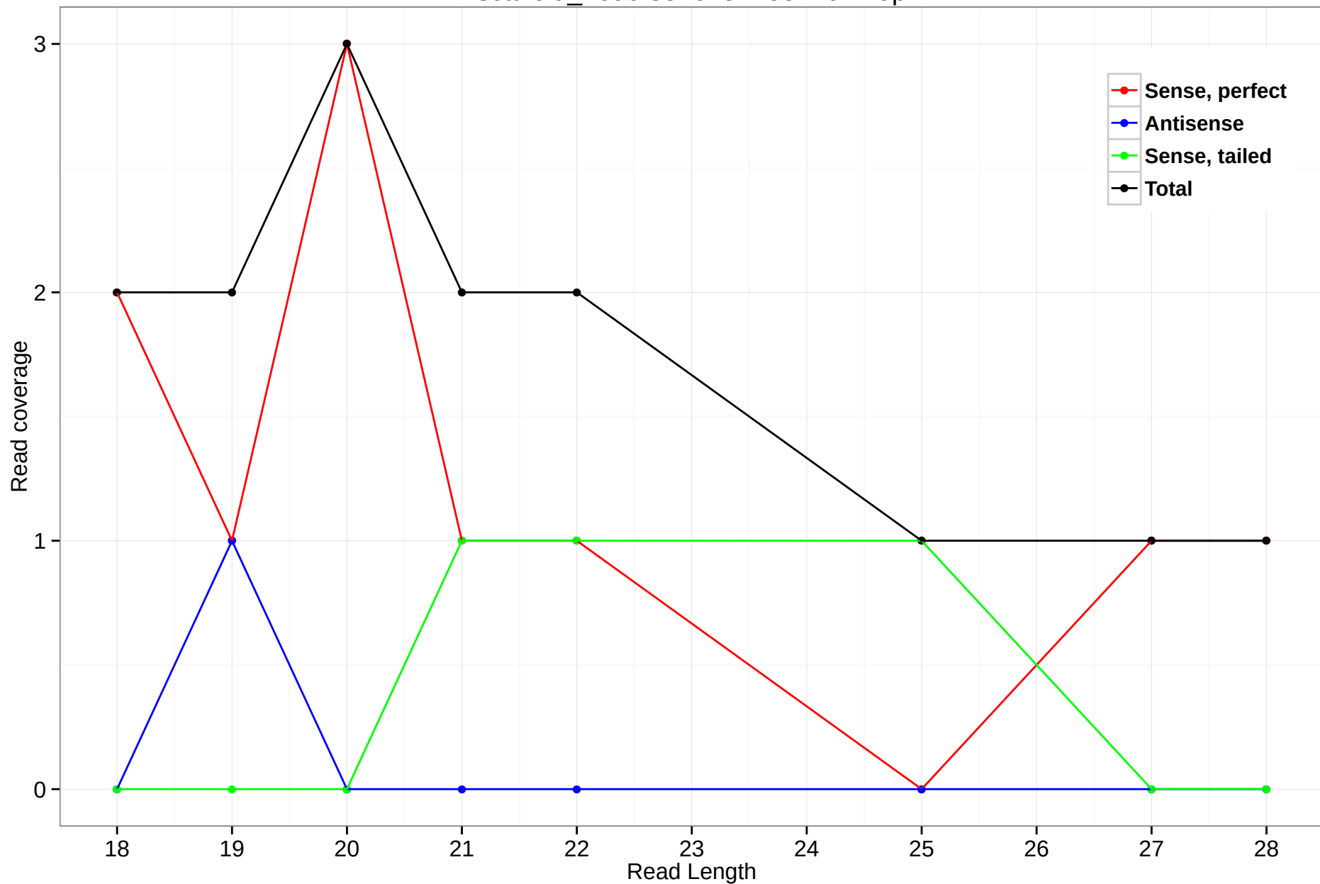
scaffold_4690:3846481-3847627.5p
