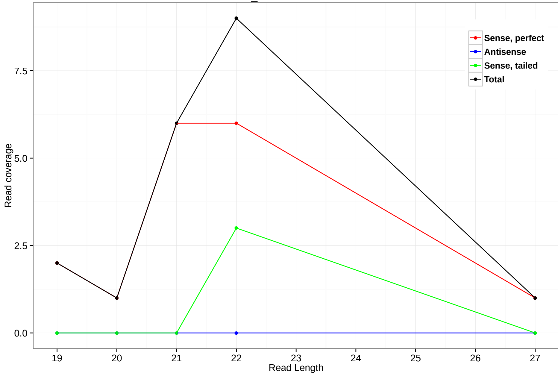
scaffold_4690:3786019-3786401
