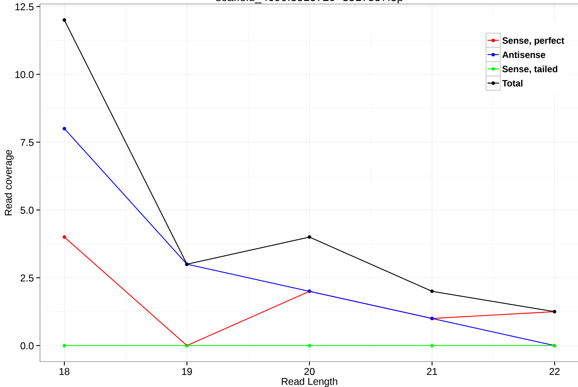
scaffold_4690:3515720-3517537.3p
