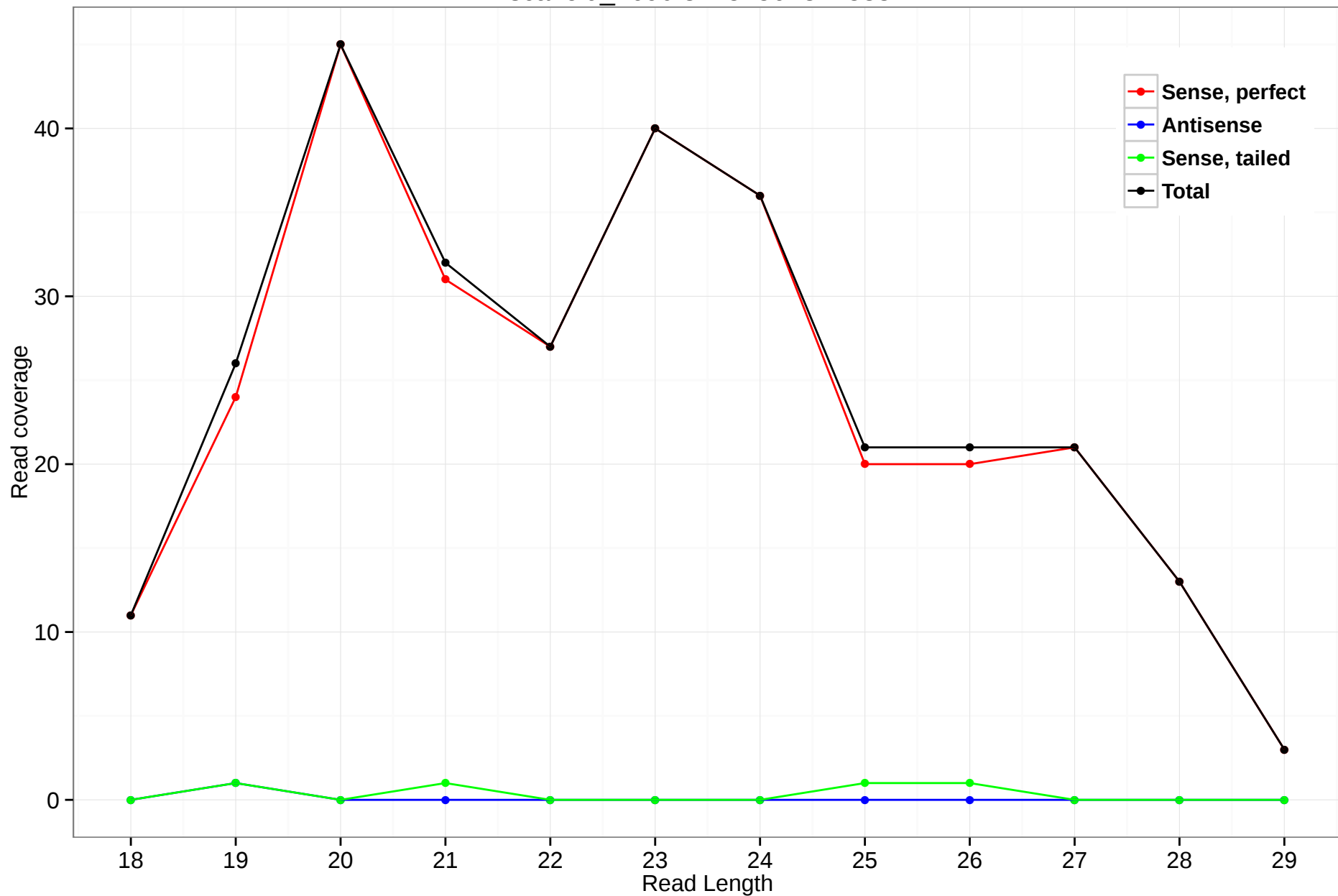
scaffold_4690:3145156-3145332
