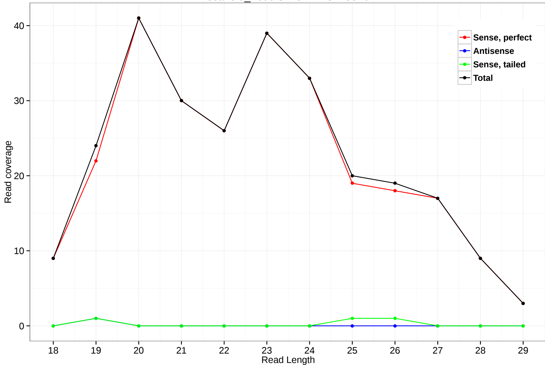
scaffold_4690:3145144-3145316
