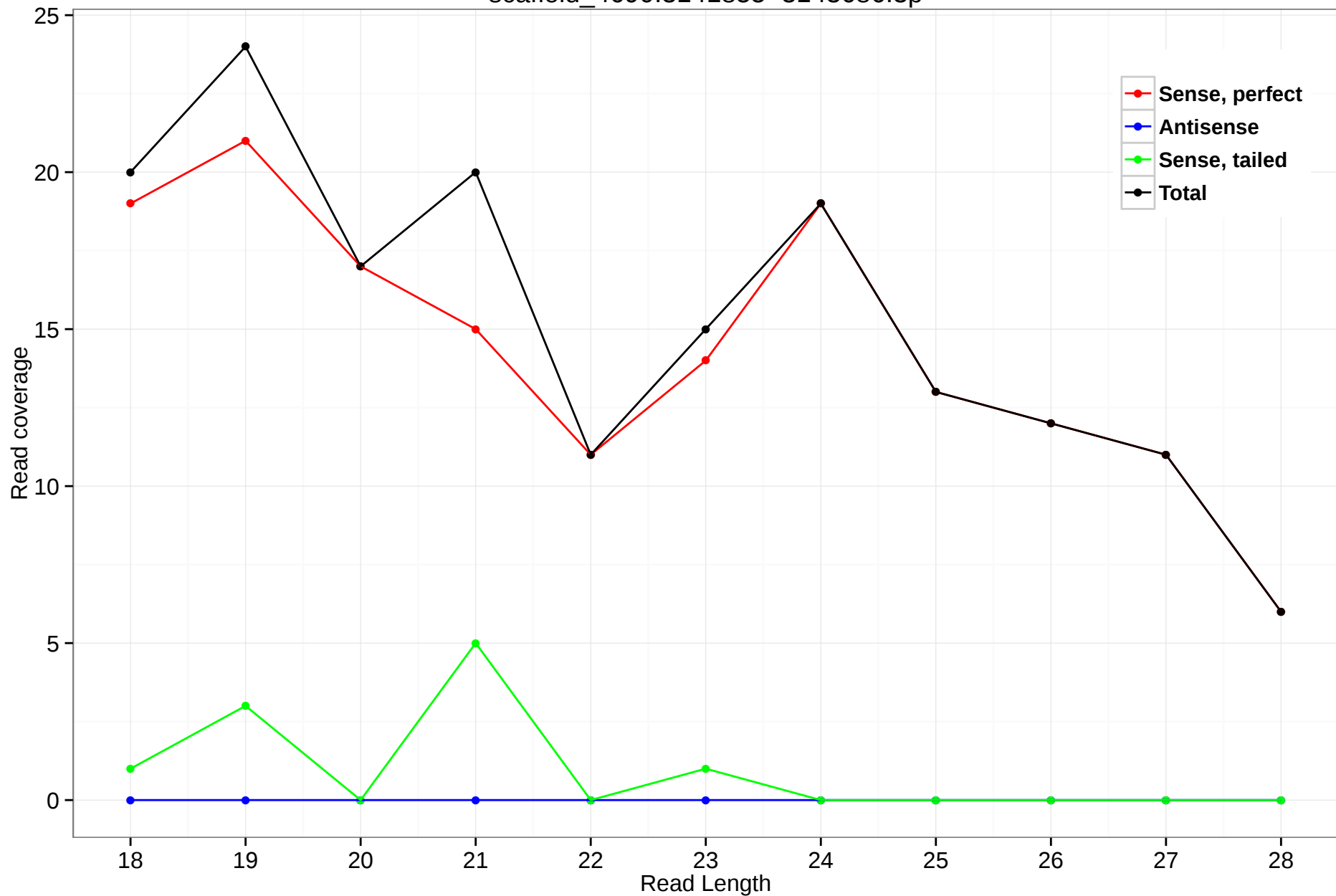
scaffold_4690:3141855-3143686.3p
