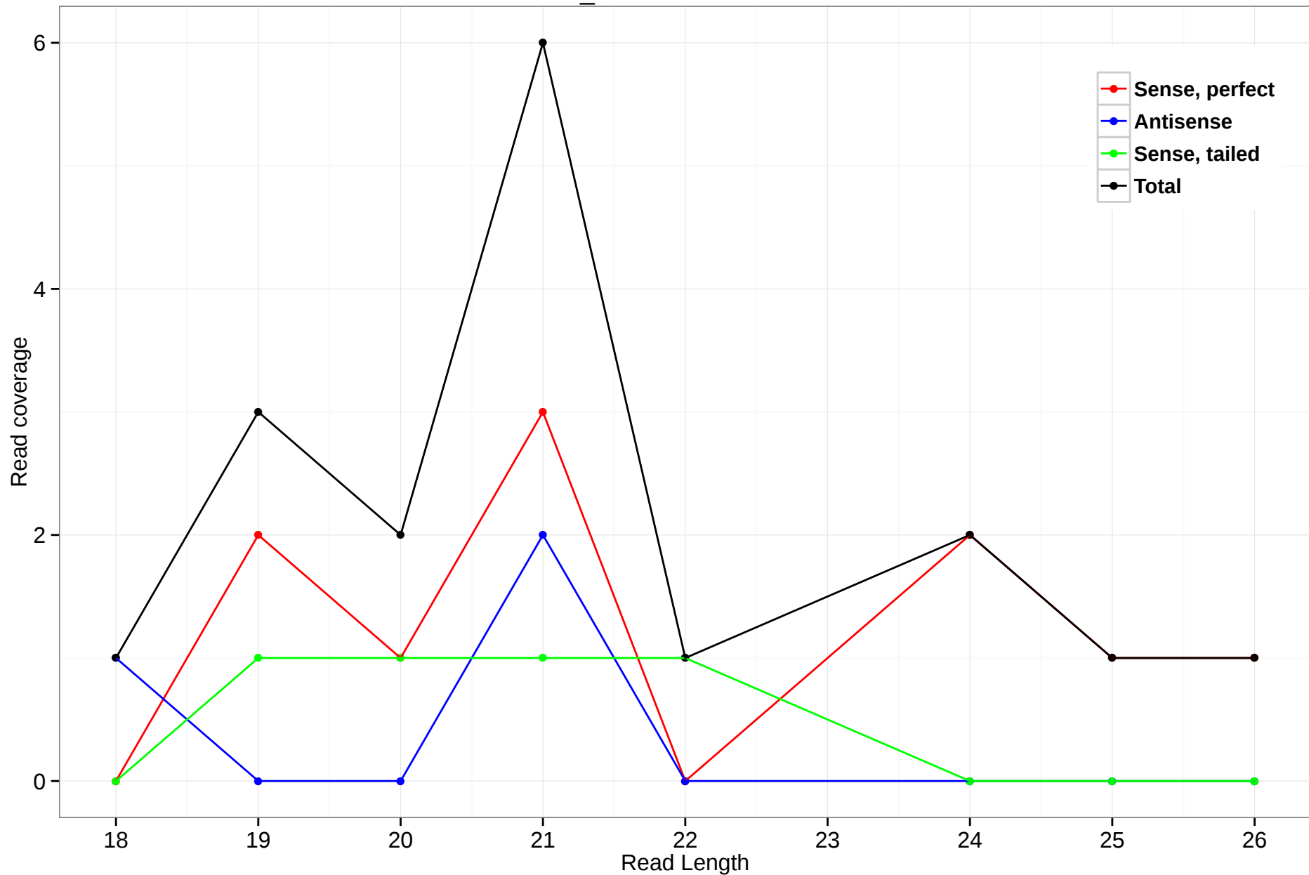
scaffold_4690:2867580-2867822
