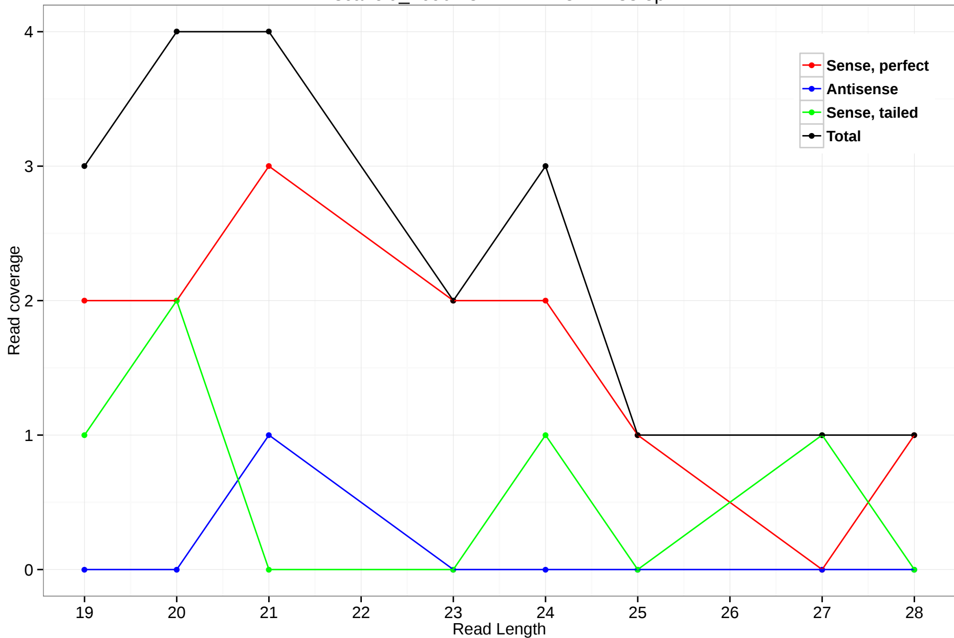
scaffold_4690:18711272-18712738.5p
