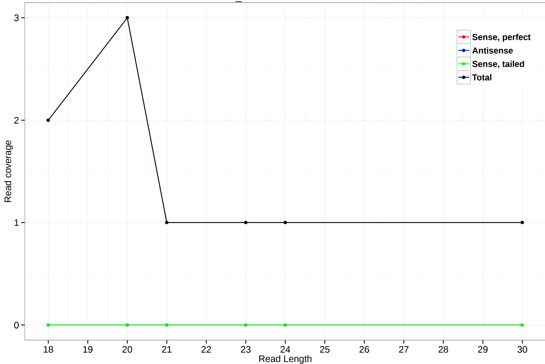
scaffold_4690:18223872-18224057
