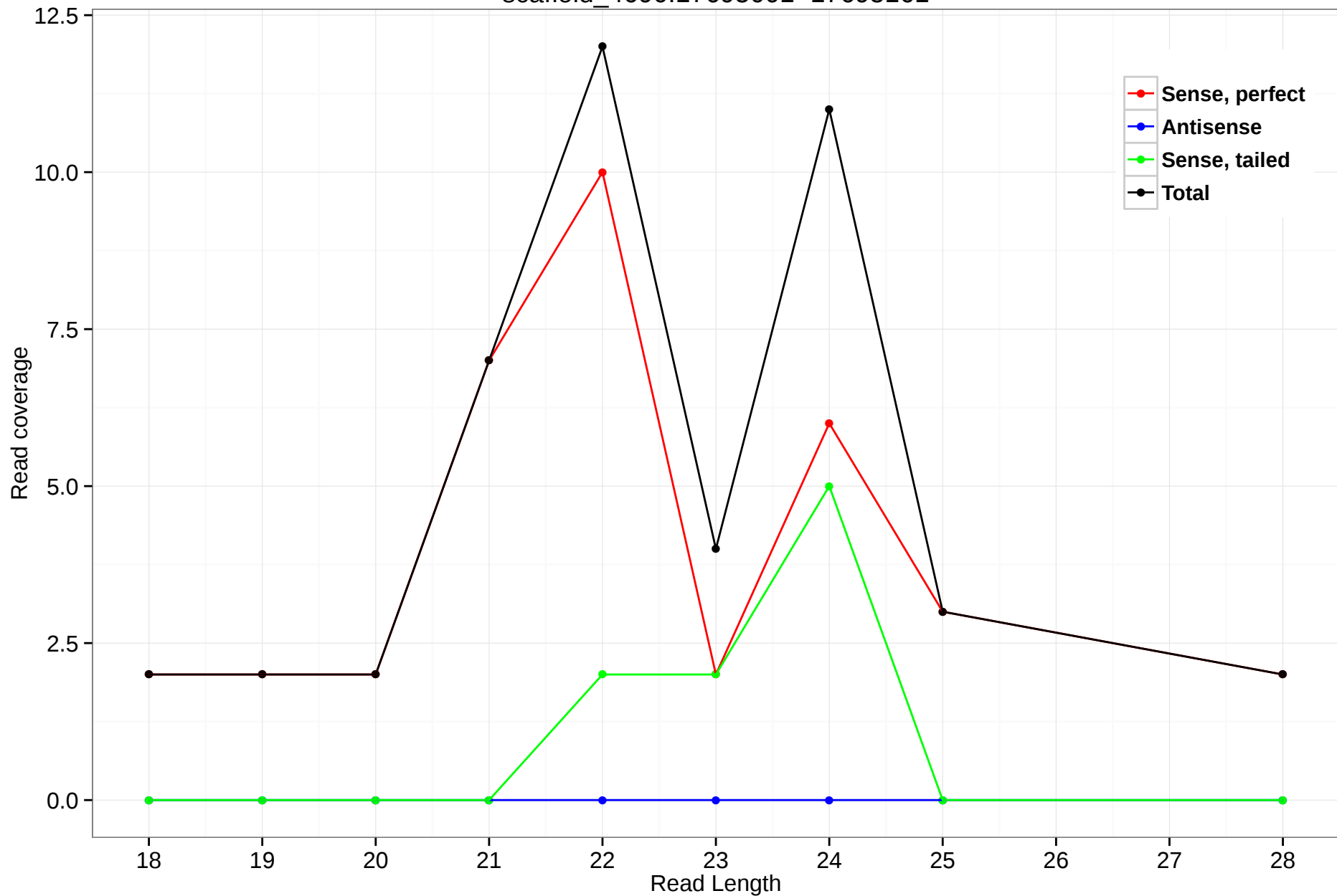
scaffold_4690:17695001-17695161
