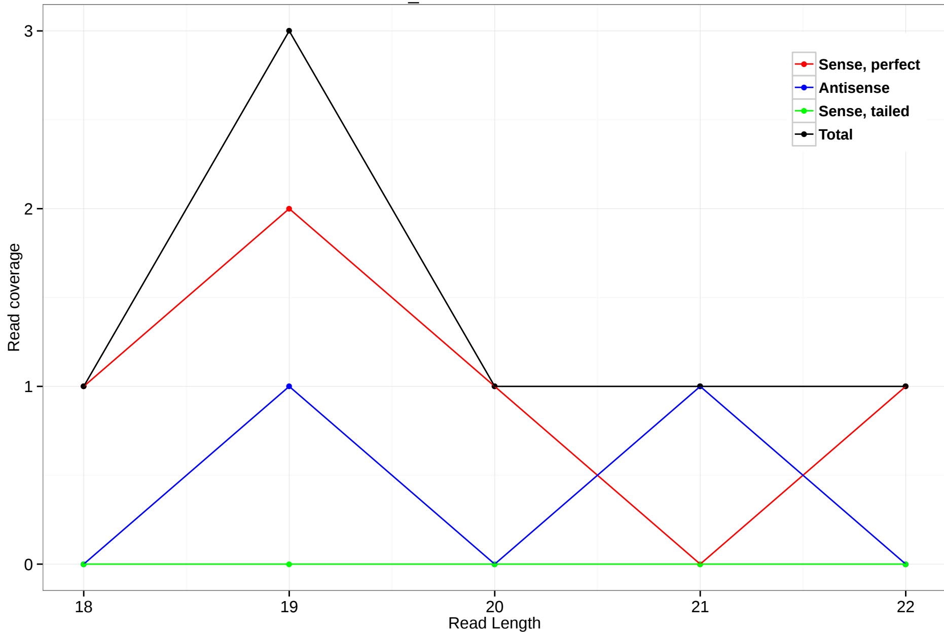
scaffold_4690:17128570-17128975
