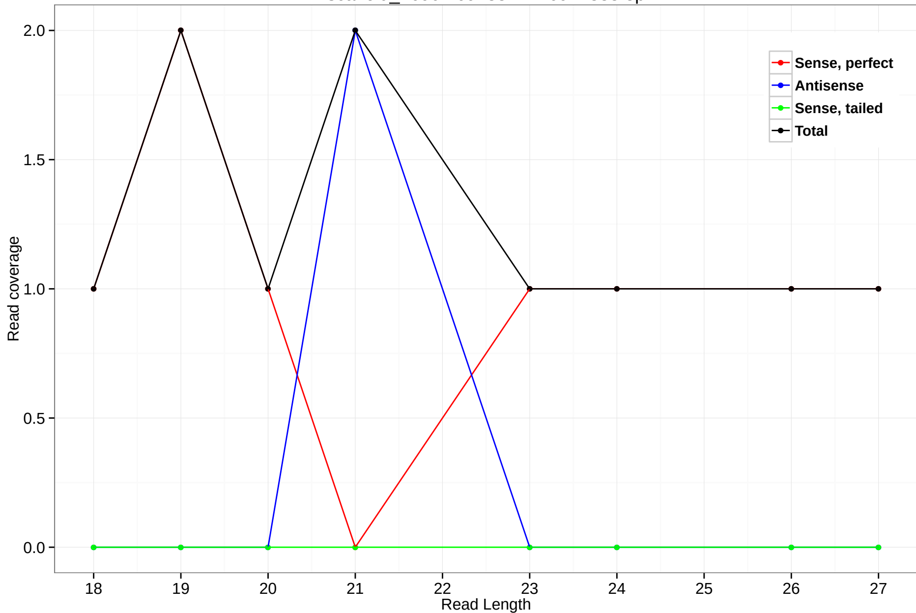
scaffold_4690:16943372-16944333.3p
