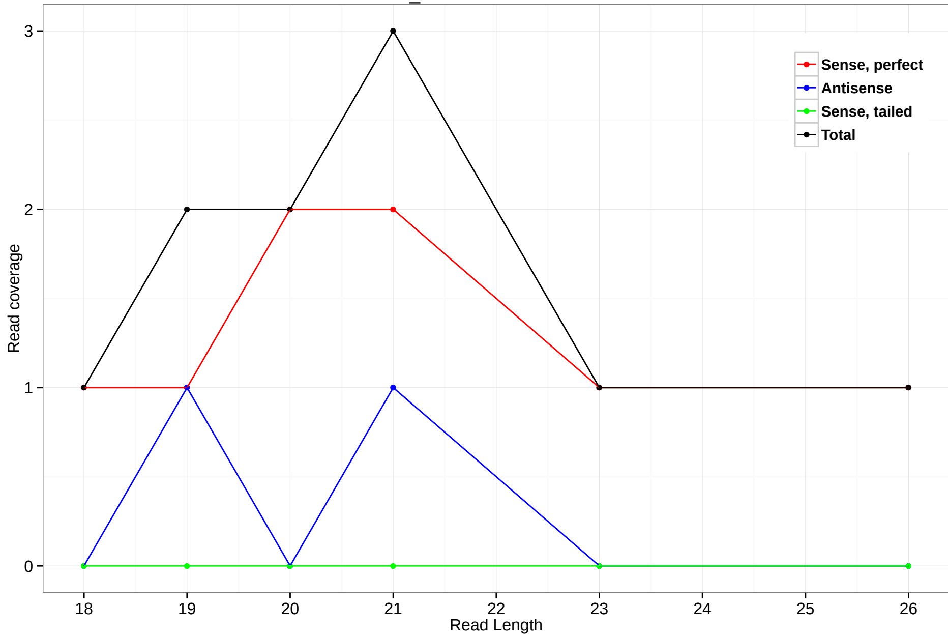
scaffold_4690:15914520-15914891
