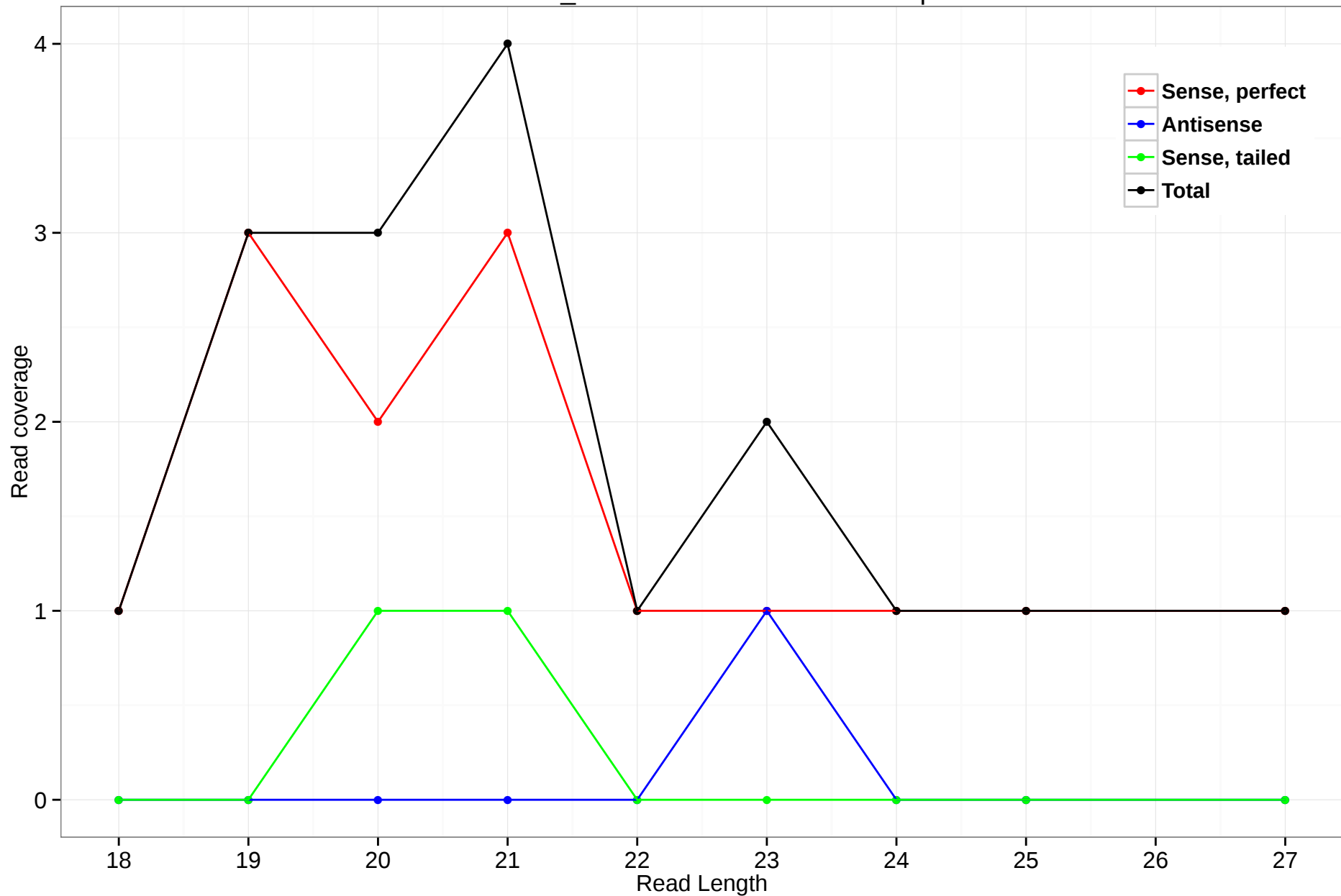
scaffold_4690:15222994-15223650.5p
