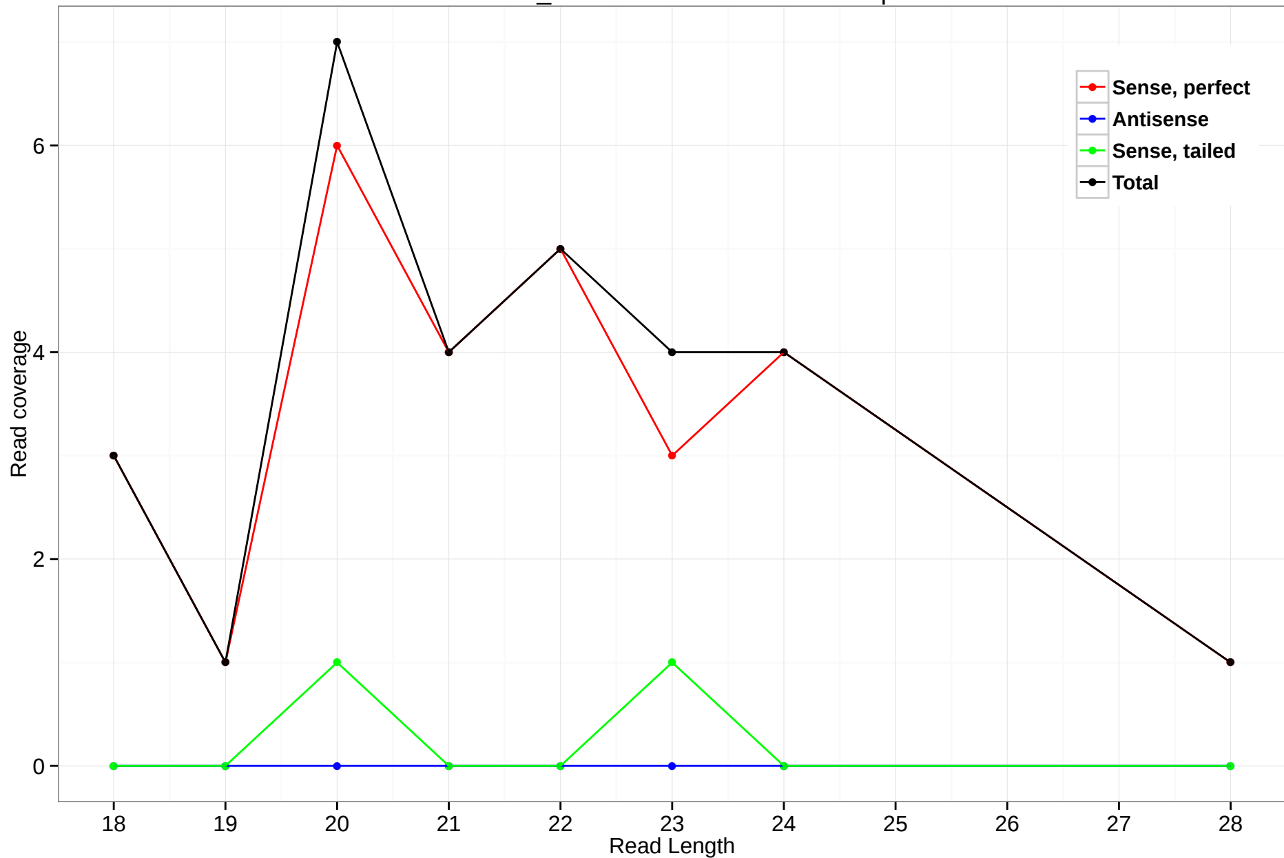
scaffold_4690:14304174-14305646.5p
