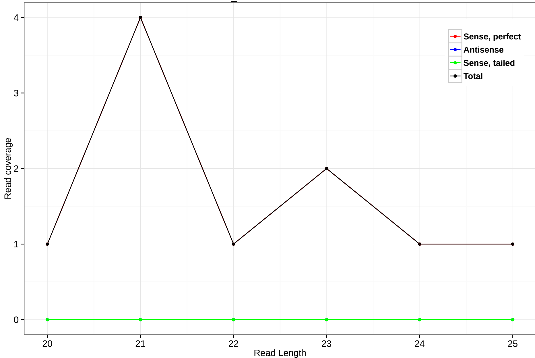
scaffold_4690:14195317-14195499
