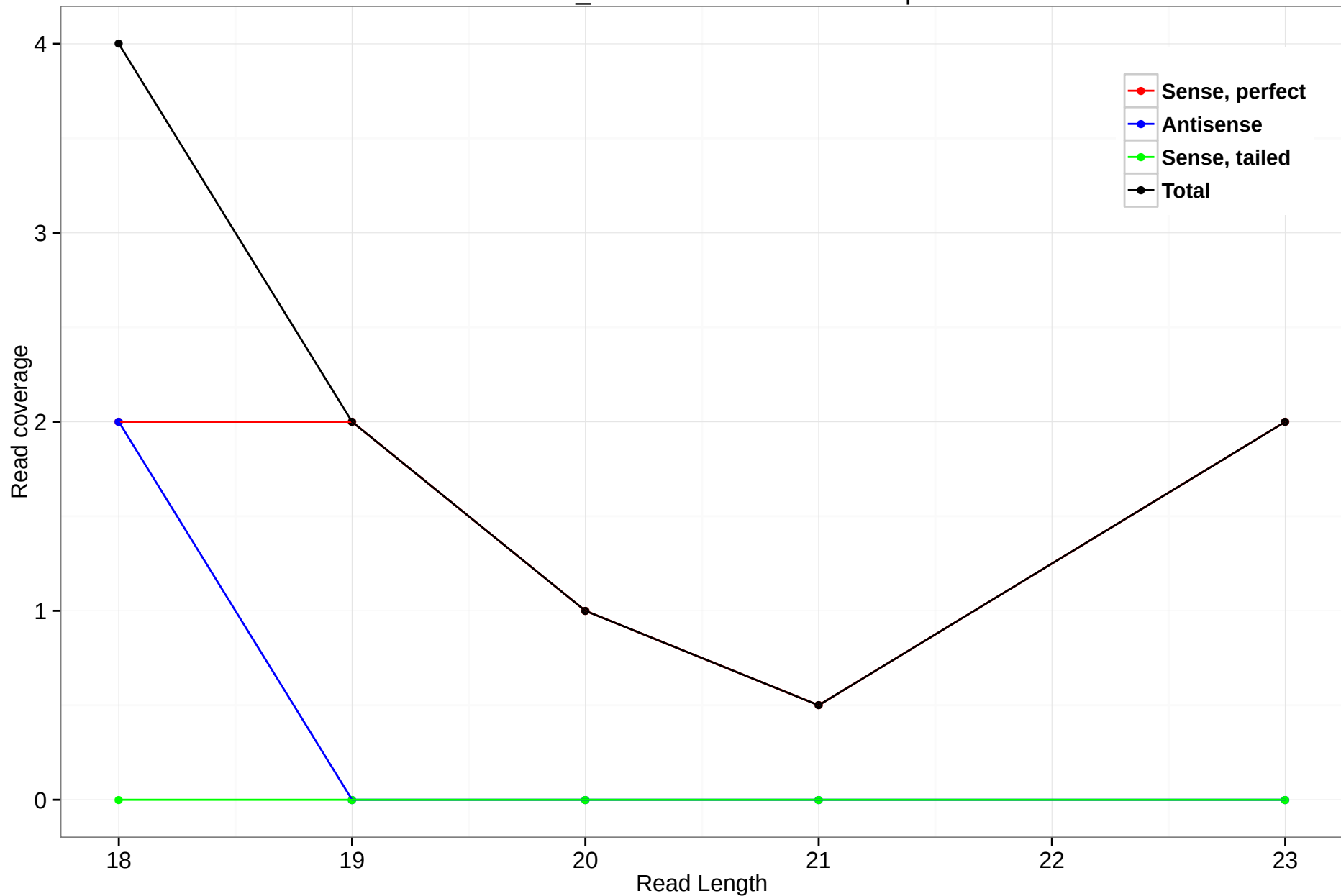
scaffold_4690:1387969-1388816.5p
