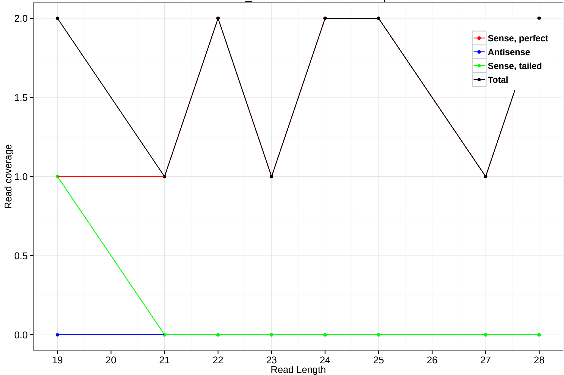
scaffold_4690:1225397-1229427.5p
