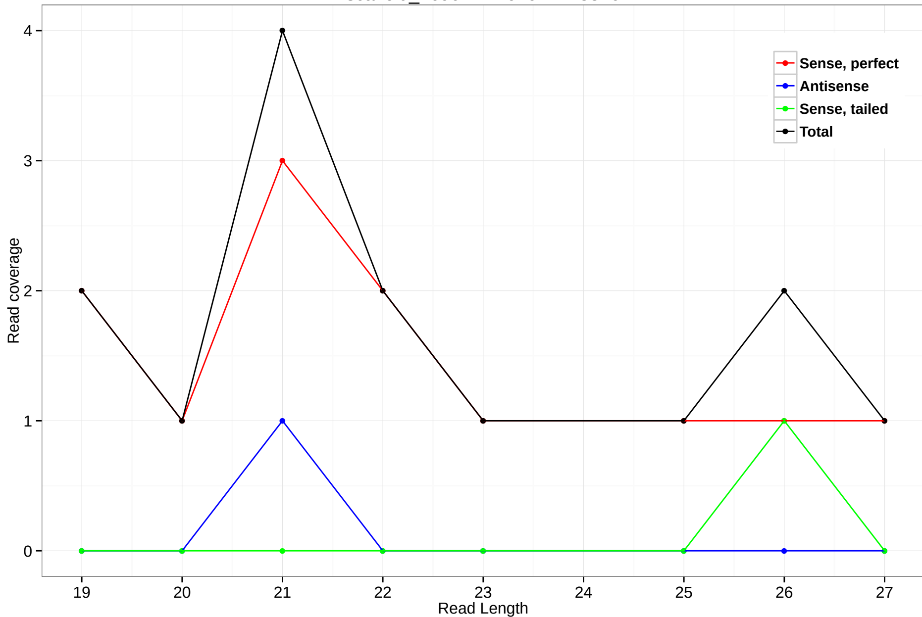
scaffold_4690:1224929-1225376
