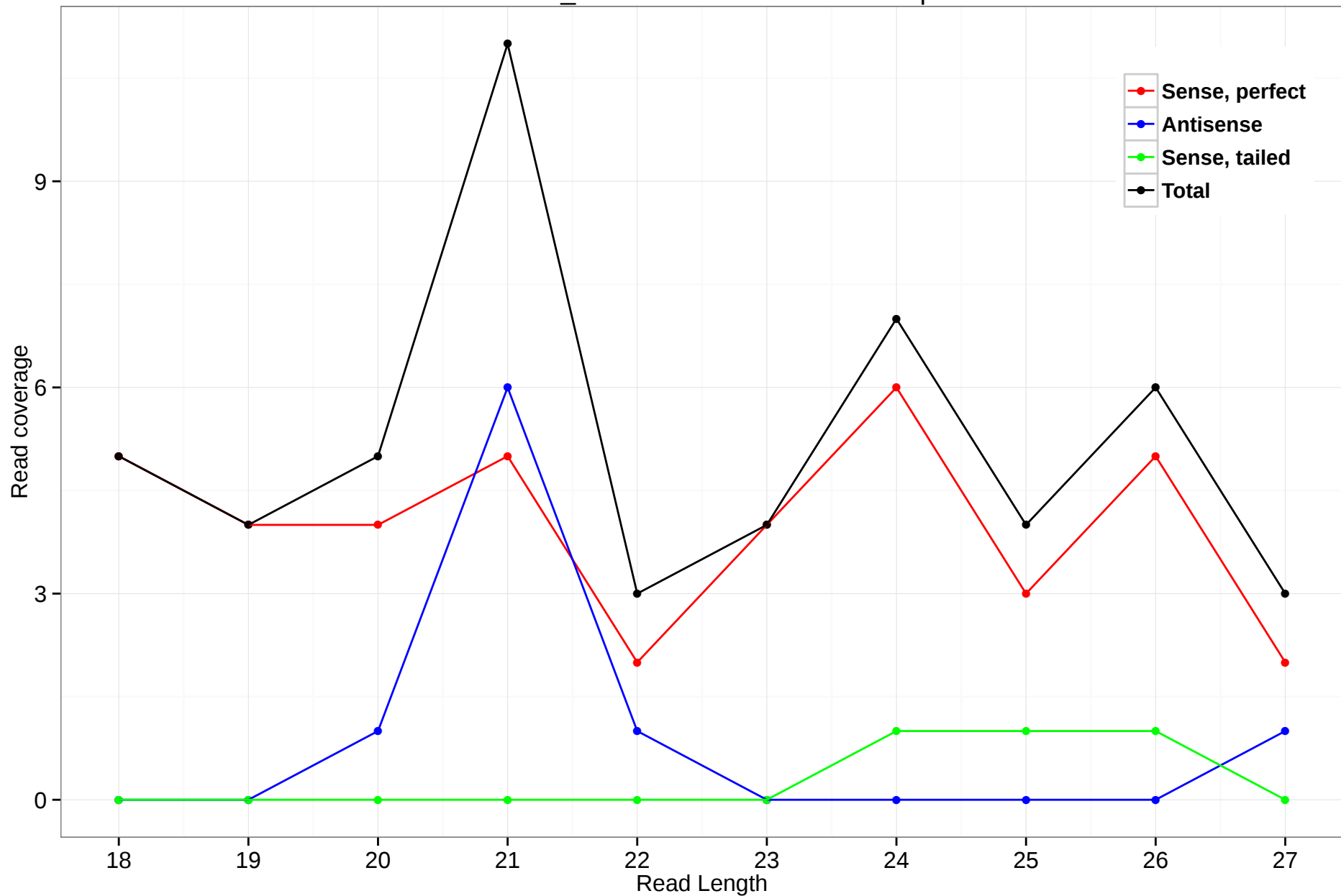
scaffold_4690:12127816-12146782.5p
