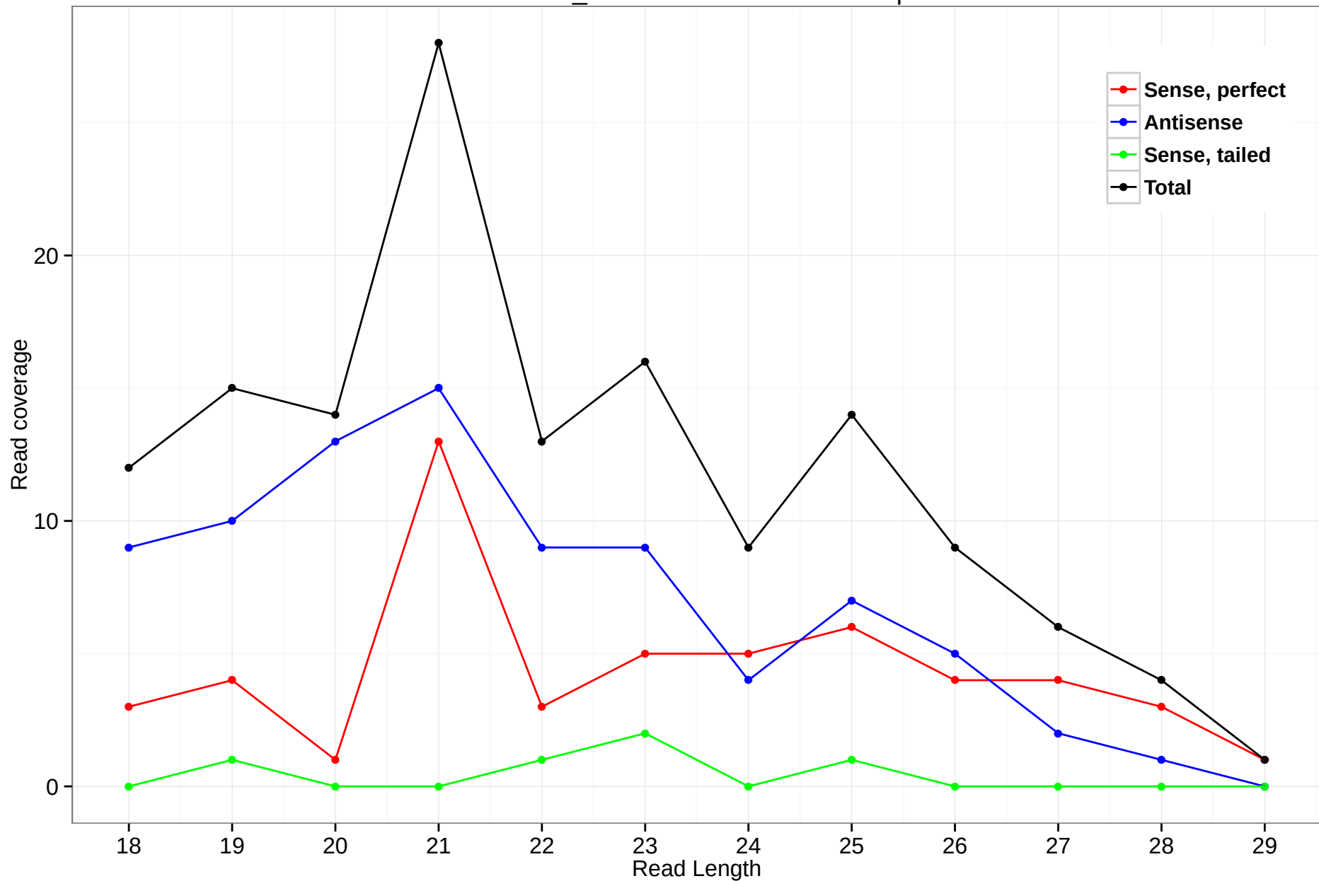
scaffold_4690:1187841-1189021.5p
