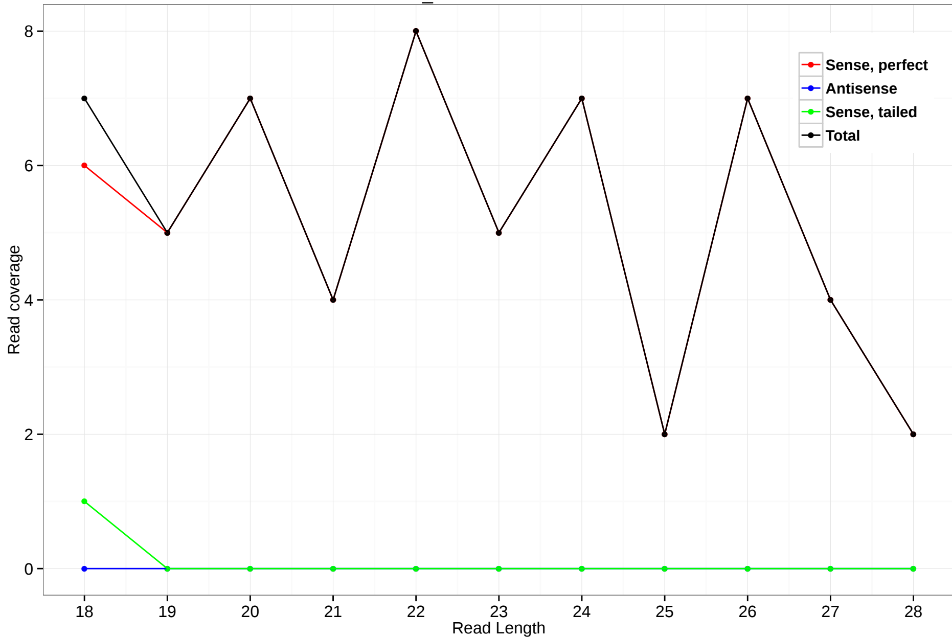
scaffold_4690:1158973-1159442
