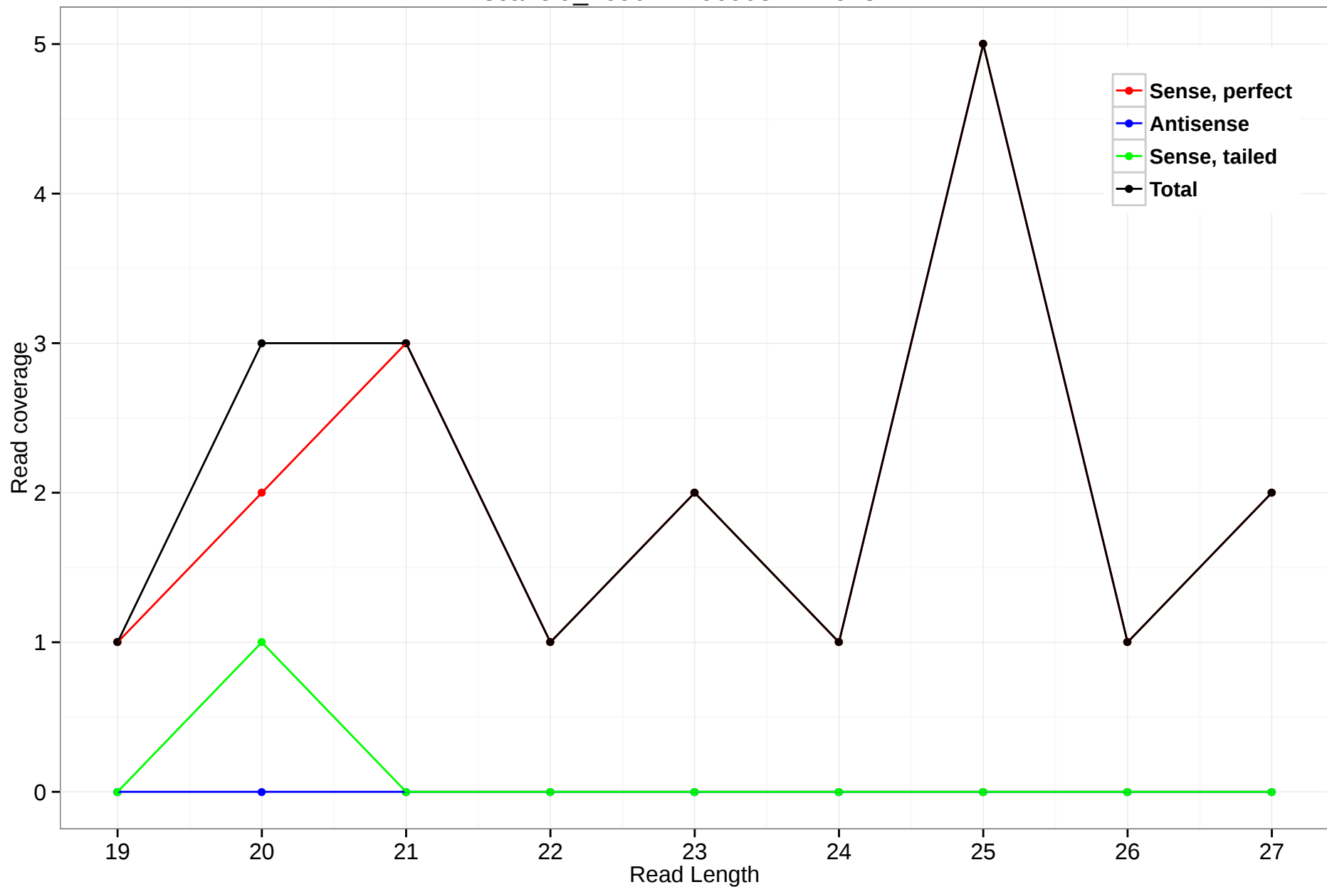
scaffold_4690:11166905-11167324
