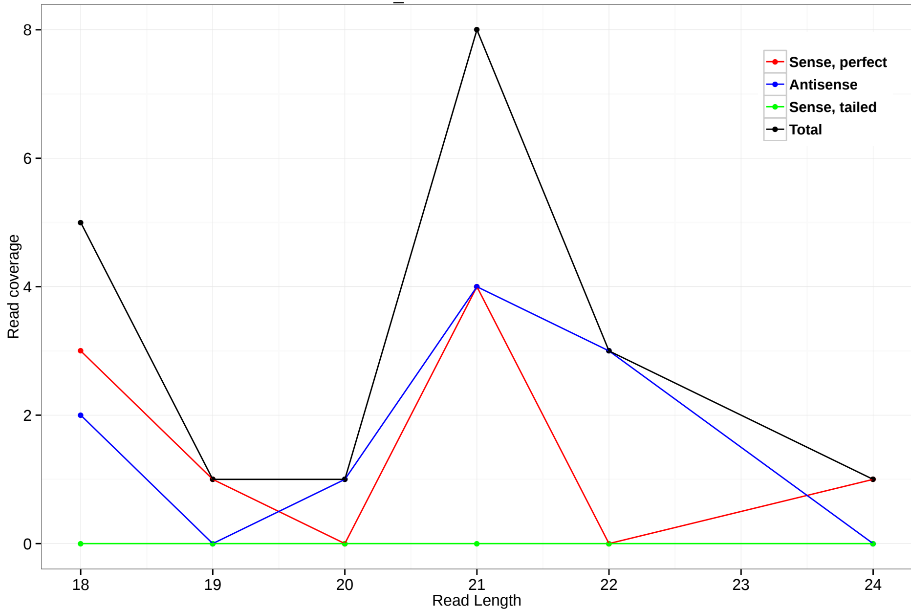
scaffold_4690:11110158-11110527
