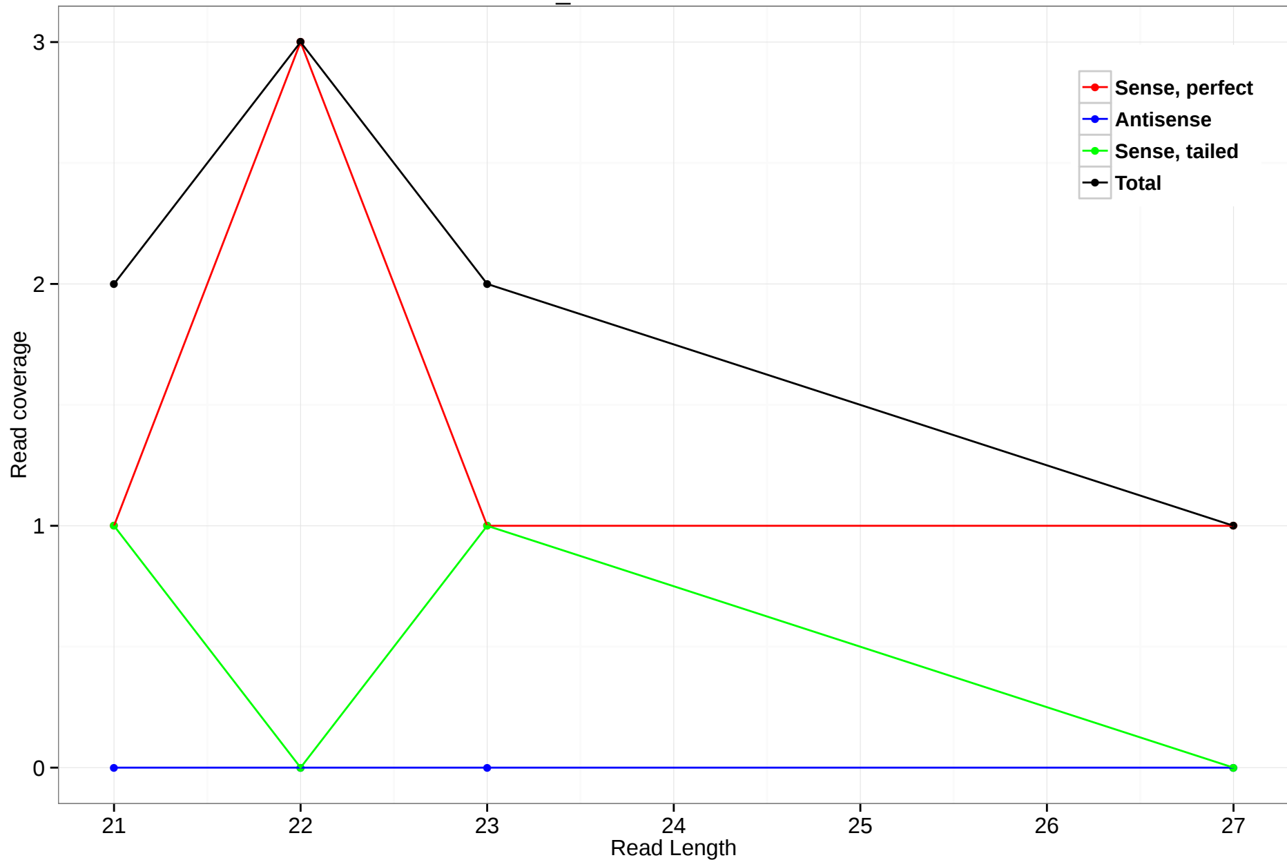
scaffold_4690:10851289-10851771
