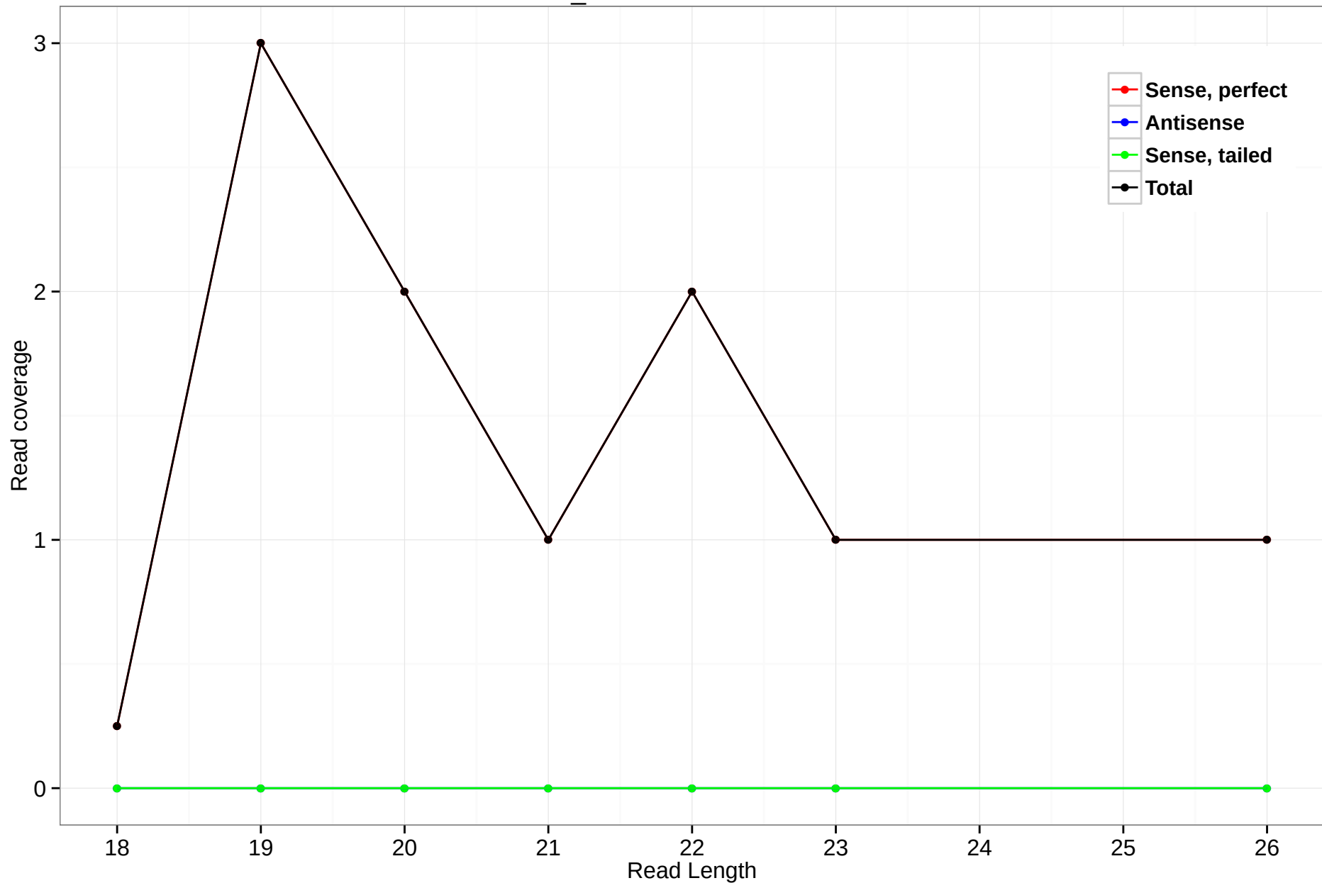
scaffold_4690:10766741-10766998
