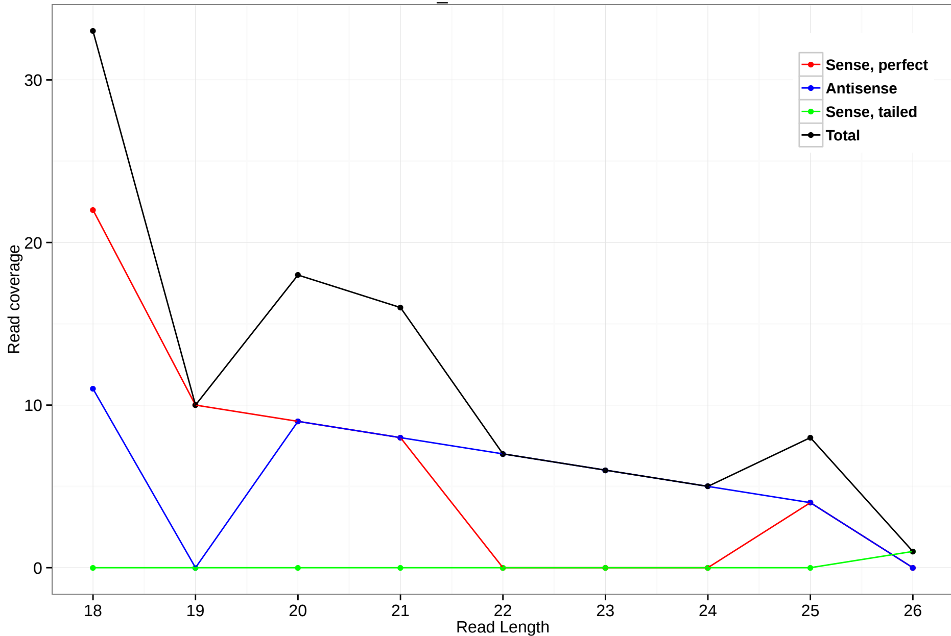
scaffold_4644:911778-912300
