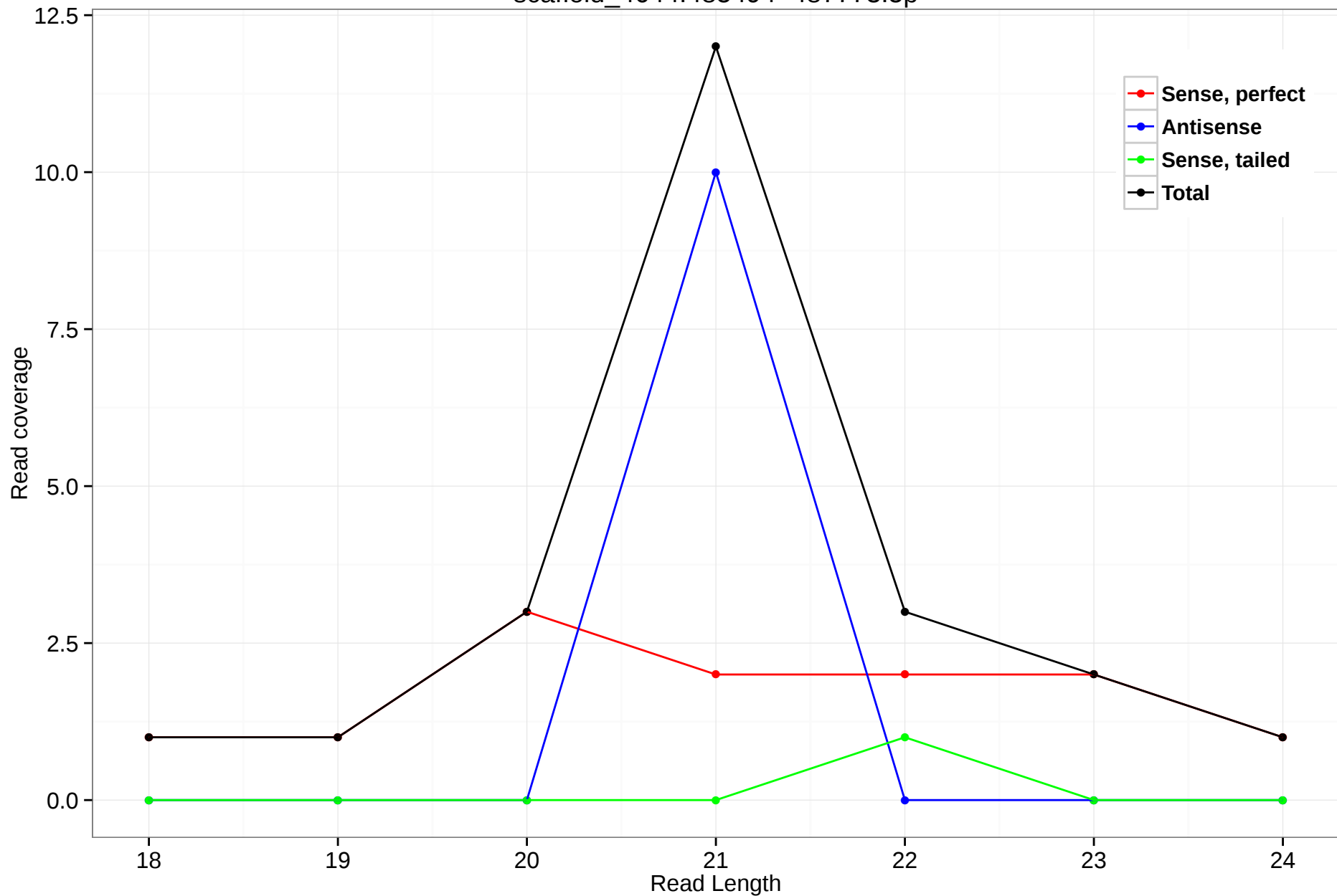
scaffold_4644:485494-487773.5p
