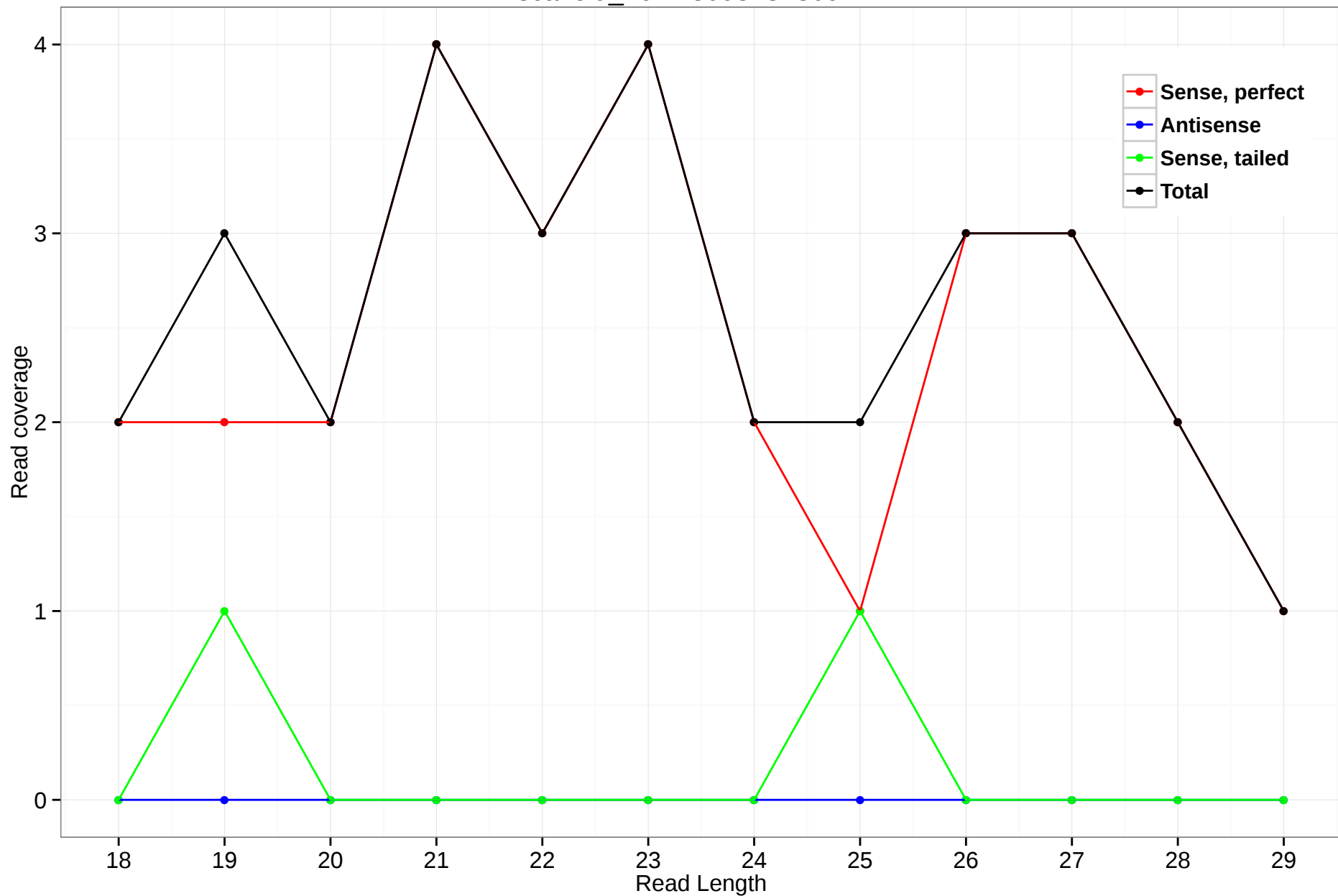
scaffold_4644:309313-309721
