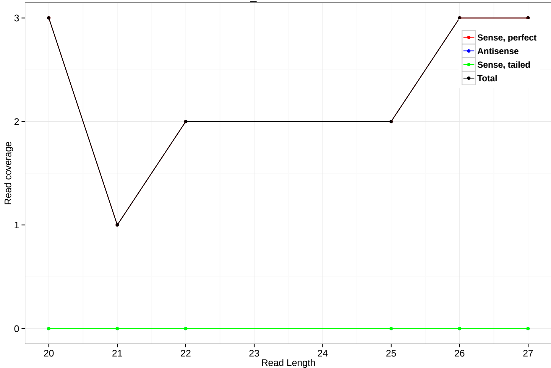
scaffold_4512:928208-928457
