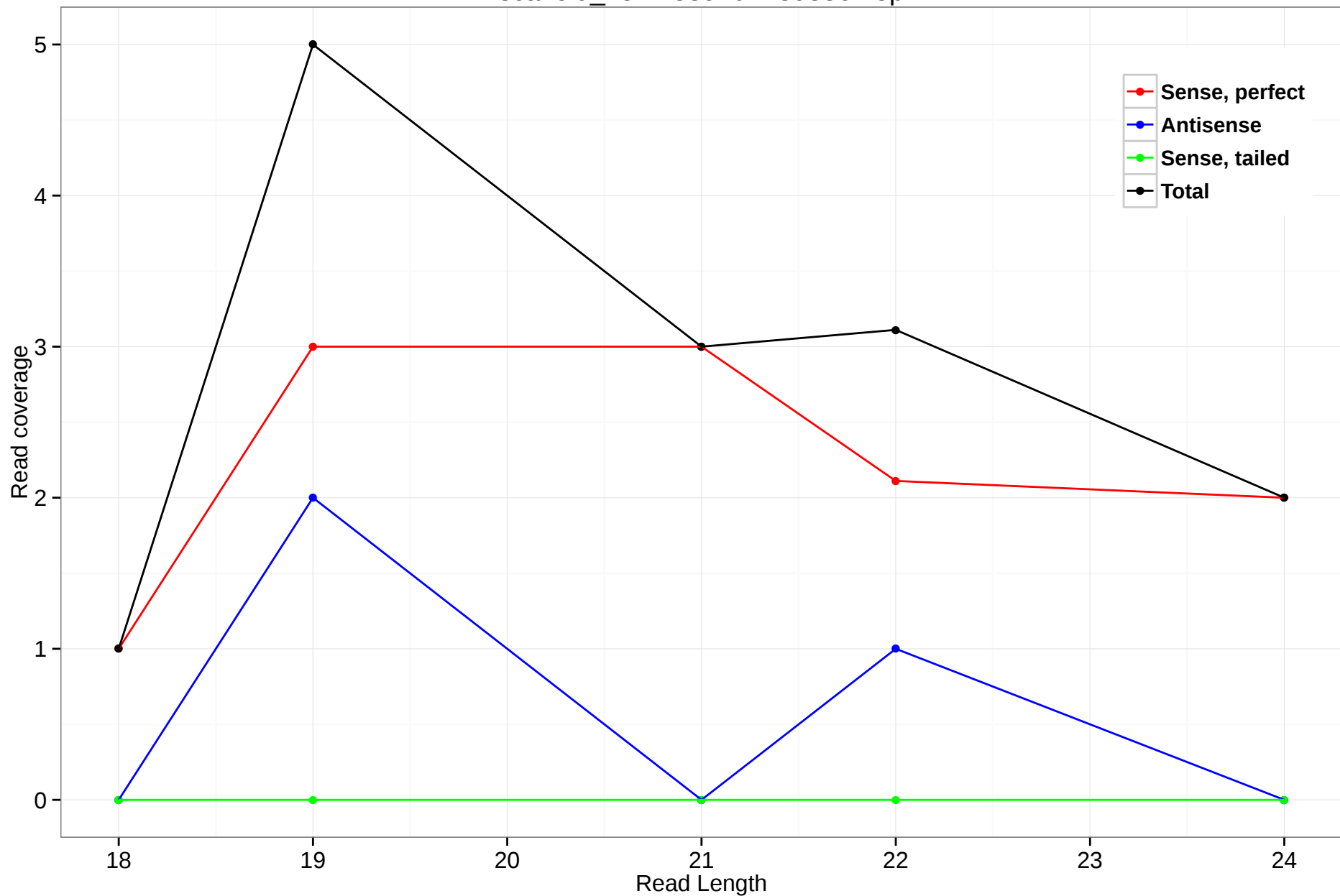
scaffold_4512:889202-893867.5p
