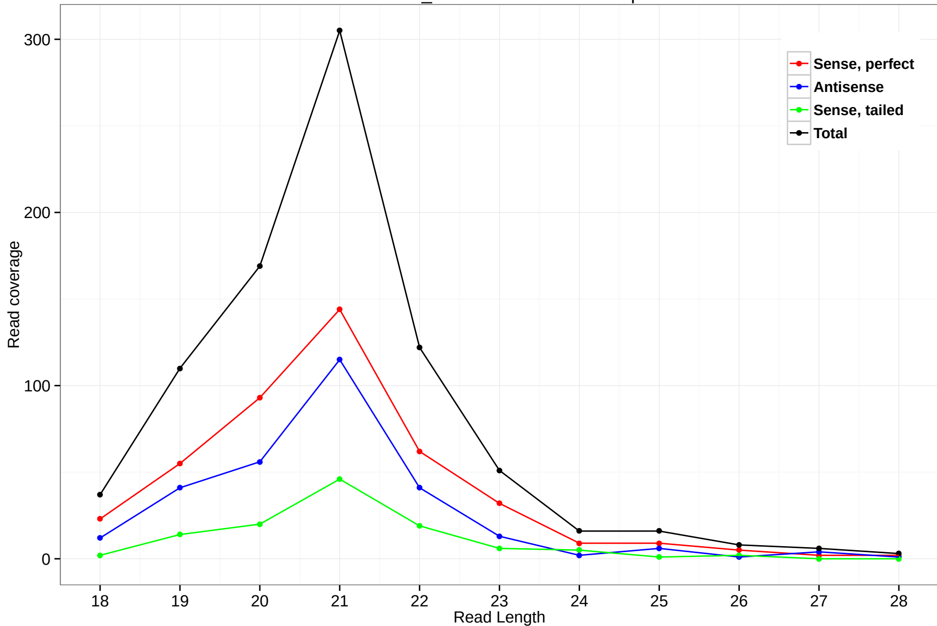
scaffold_4512:590451-593215.5p
