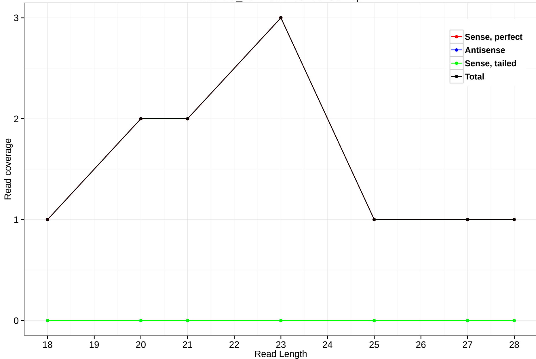
scaffold_4512:550786-551397.3p
