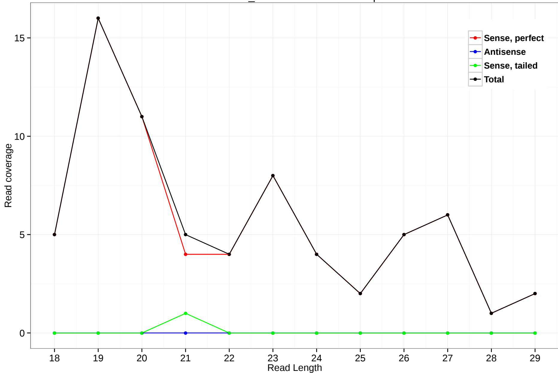
scaffold_4512:167705-168873.5p
